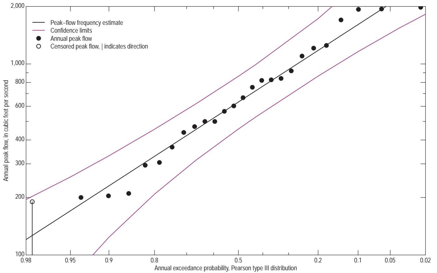
05476989 East Fork Des Moines River above Ceylon, Minn.
