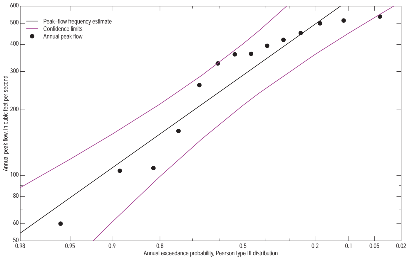
06482500 North Branch Pipestone Creek near Pipestone, Minn.
