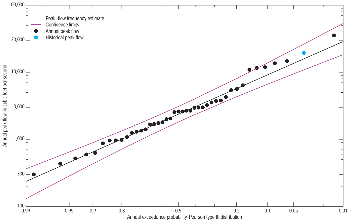
06483000 Rock River at Luverne, Minn.
