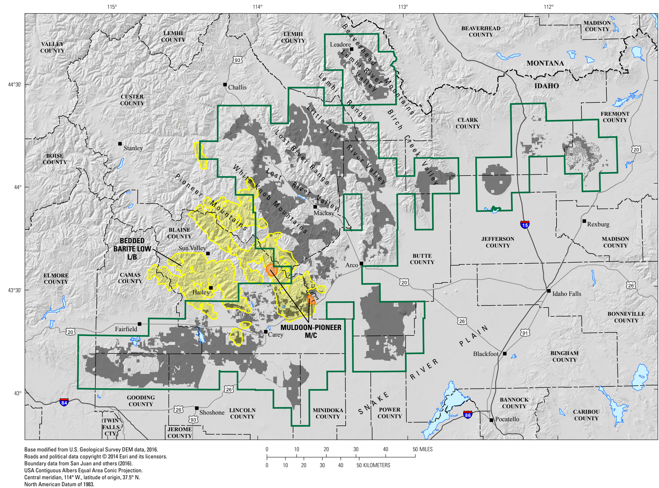
Figure 28. Map showing mineral-resource potential for bedded barite-type deposits in the study area for the North-Central Idaho Sagebrush Focal Area.
