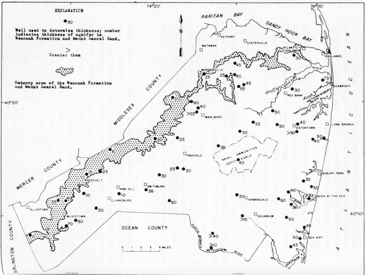
Figure 19.—Thickness of the aquifer in the Wenonah Formation and Mount Laurel Sand.
