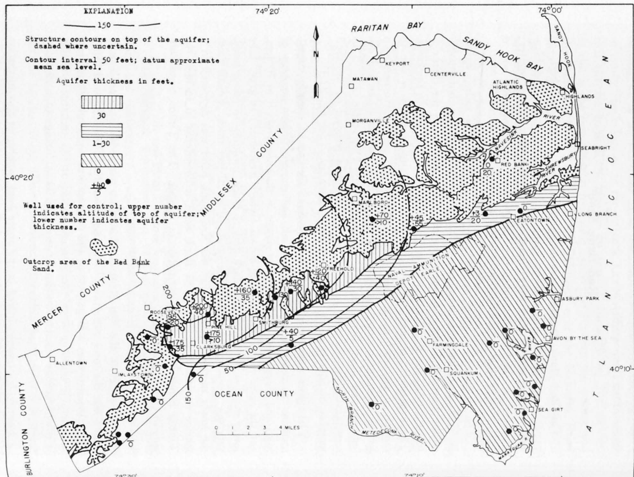
Figure 22.—Structure contours on top of the aquifer of the Red Bank Sand and thickness of the aquifer.
