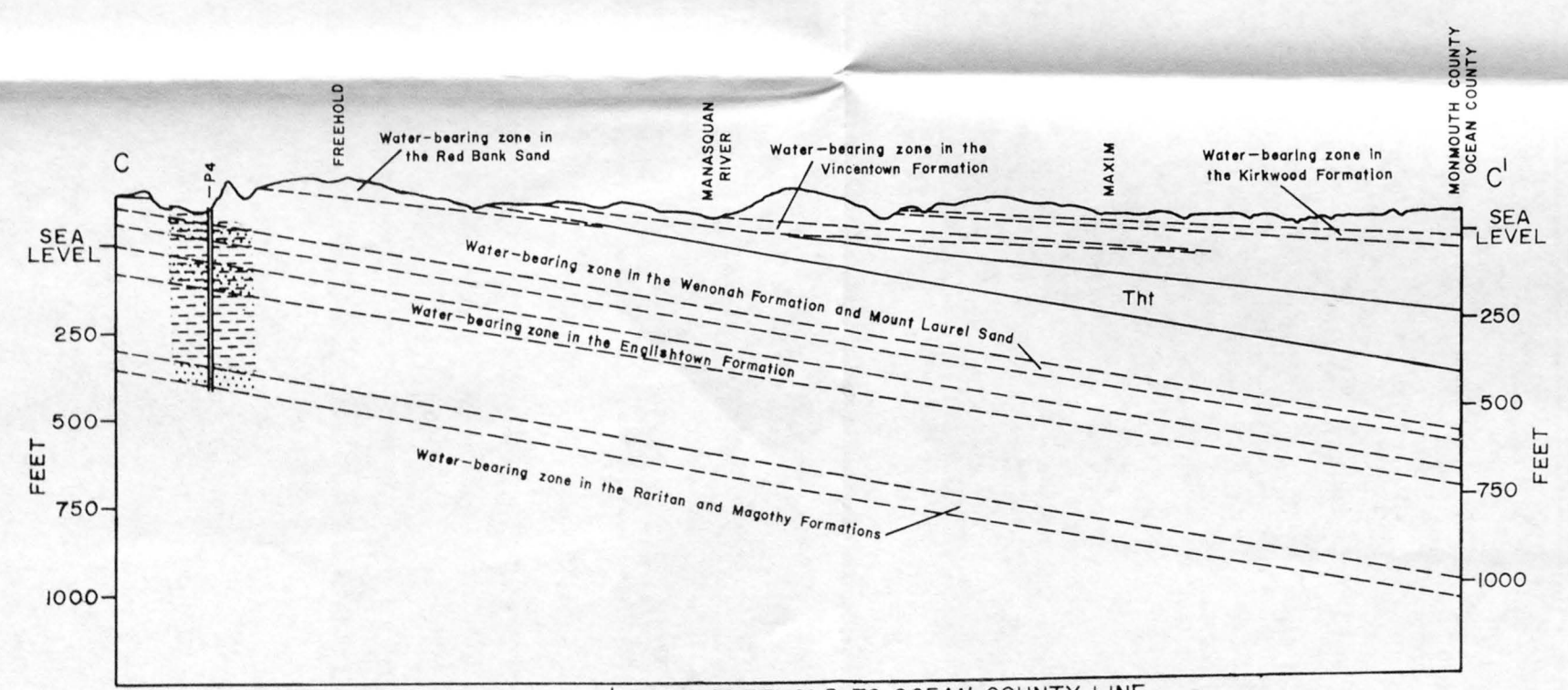
SECTION C-C' FROM FREEHOLD TO OCEAN COUNTY LINE
