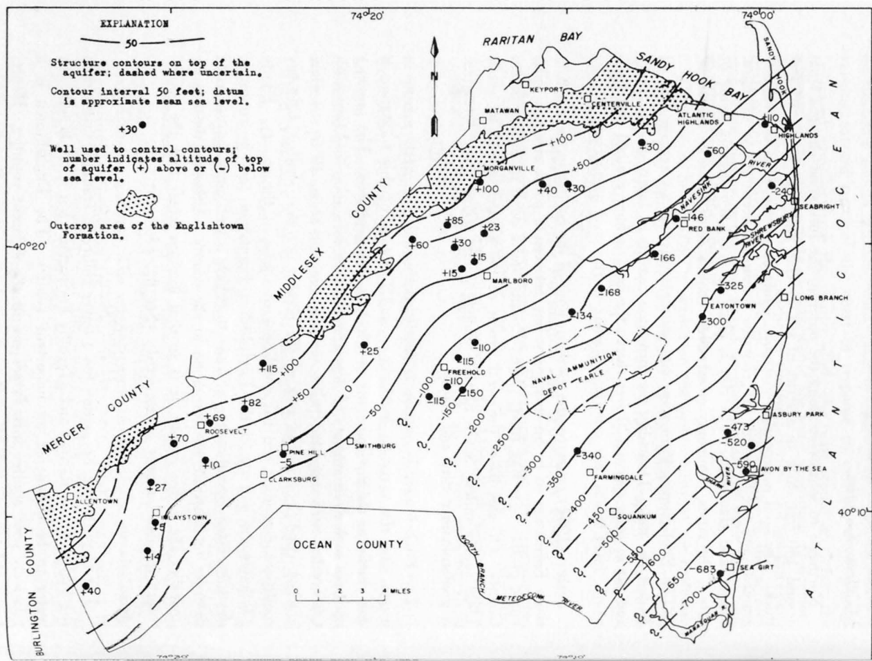
Figure 12.—Structure contours on top of the aquifer in the Englishtown Formation.
