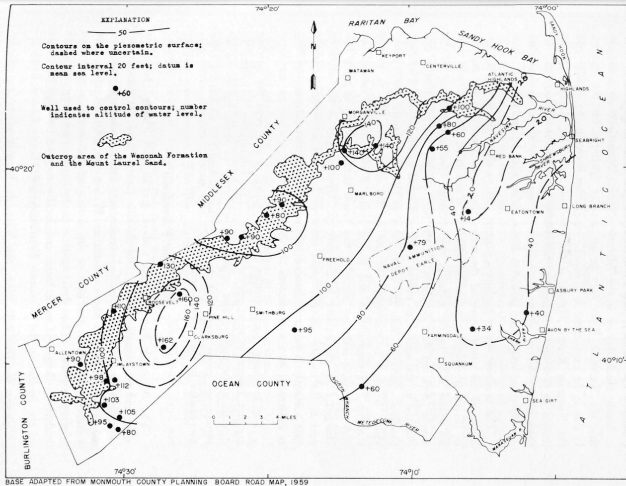
Figure 21.—Contours on the piezometric surface of the Wenonah Formation and Mount Laurel Sand, January 1959.
