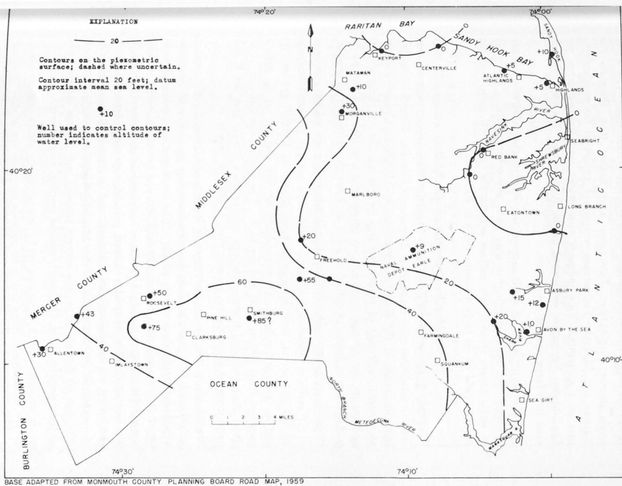
Figure 11.—Contours on the piezometric surface of the Raritan and Magoghy Formations for a selected period in 1959.
