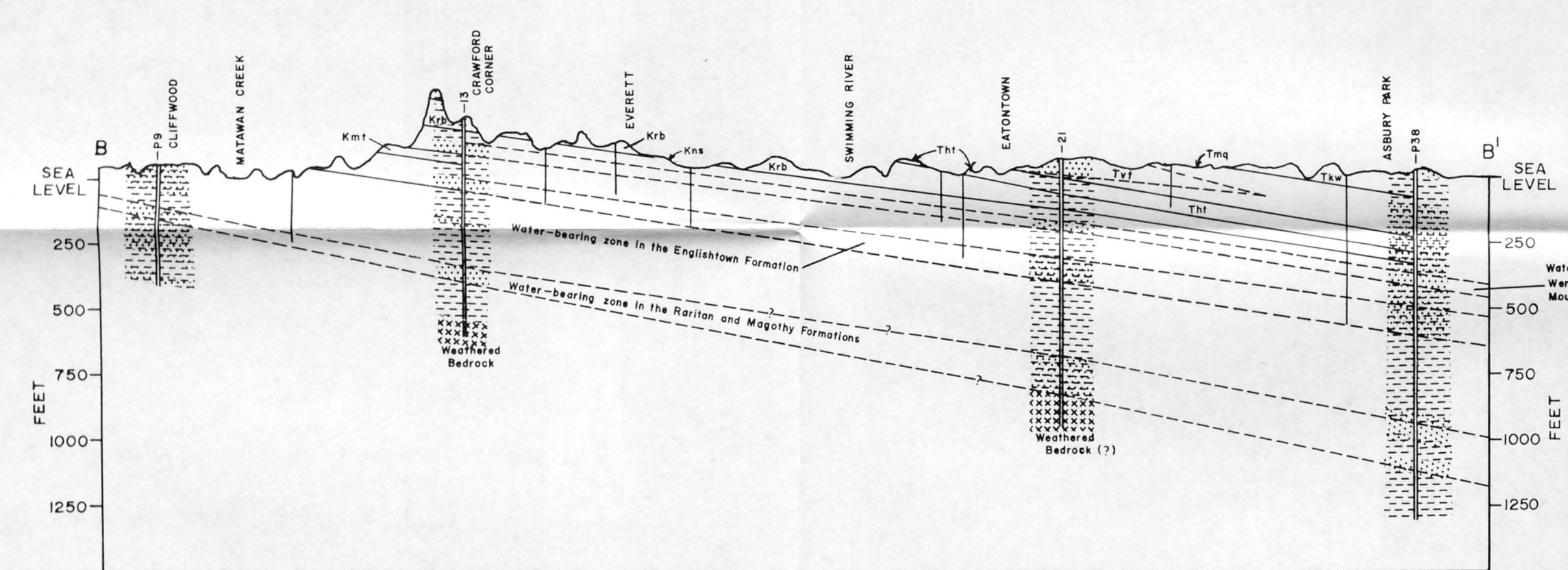
SECTION B-B' FROM CLIFFWOOD THROUGH ASBURY PARK
