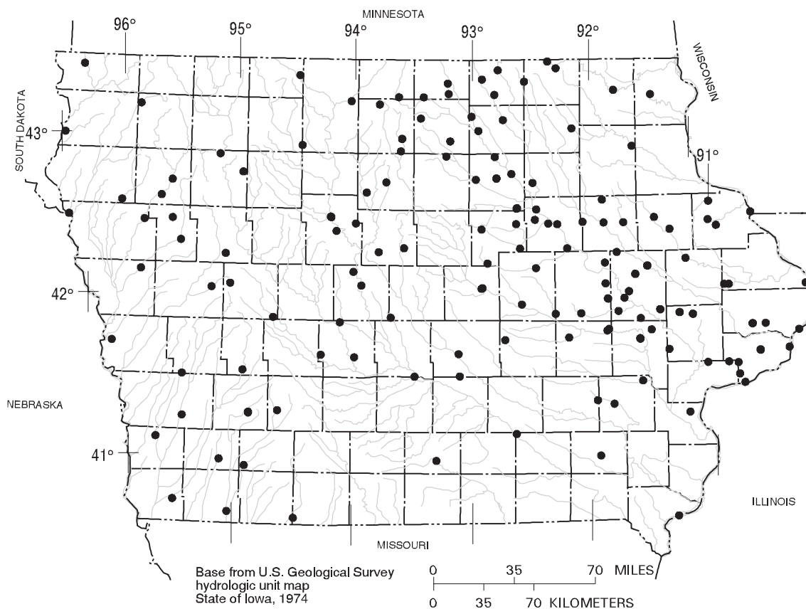
Figure 3. Location of active ground-water-quality monitoring wells, water year 2004.
