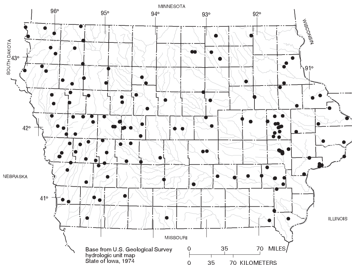
Figure 2. Location of wells in the ground-water-level observation network, water year 2004.
