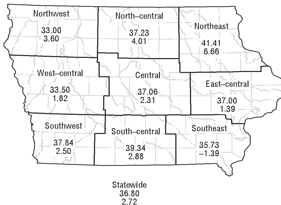
Figure 1. Water year 2004 precipitation record for the National Weather Service's designated Climatological Districts [upper value: average precipitation for the water year, in inches; lower value: deviation from long-term average (1971-2000), in inches; source: Harry Hillaker, State Climatologist, Iowa Department of Agriculture and Land Stewardship, written commun., 2004]
