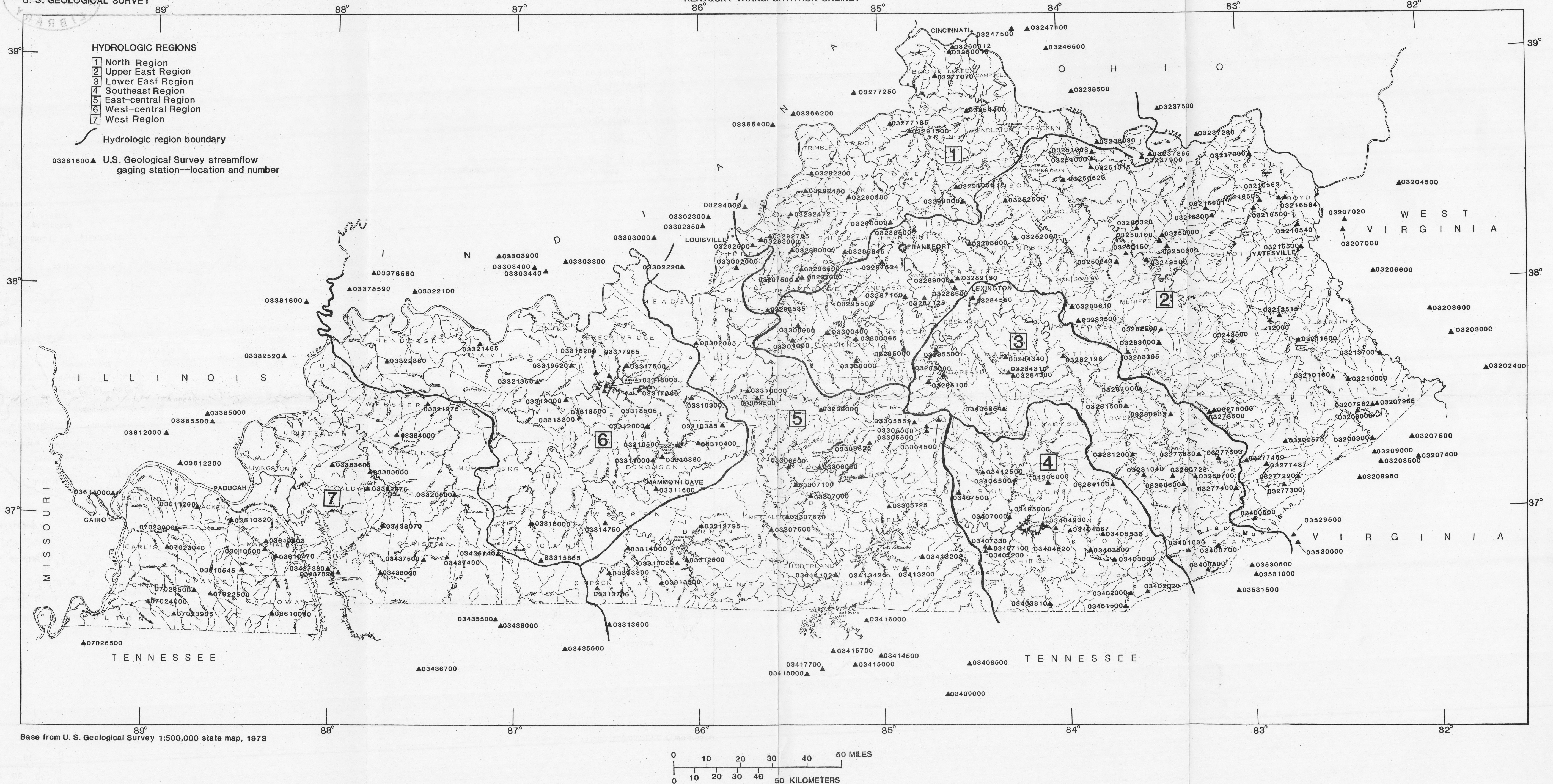
LOCATIONS OF HYDROLOGIC REGION BOUNDARIES AND STREAMFLOW GAGING STATIONS USED IN THE STUDY
