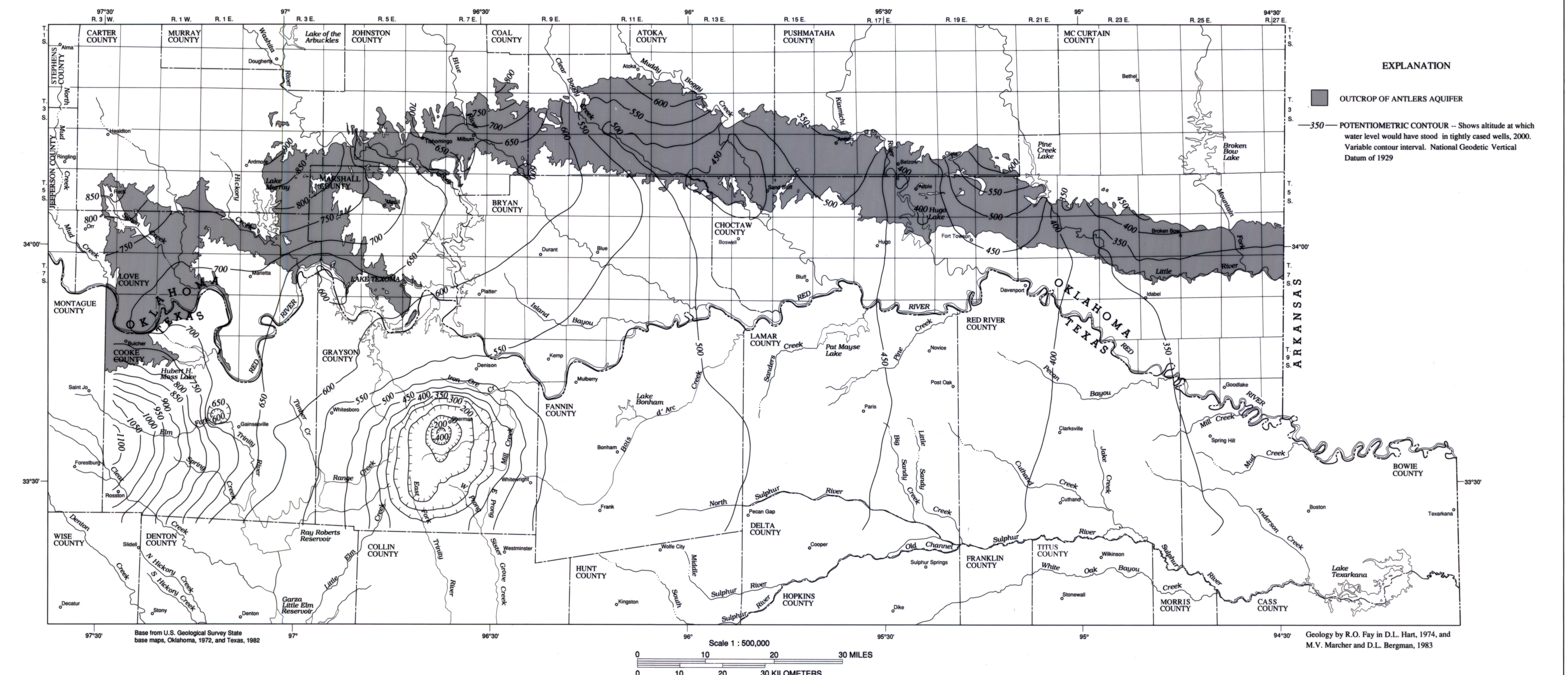
C. MAP SHOWING POTENTIOMETRIC SURFACE IN THE ANTLERS AQUIFER, 2000
