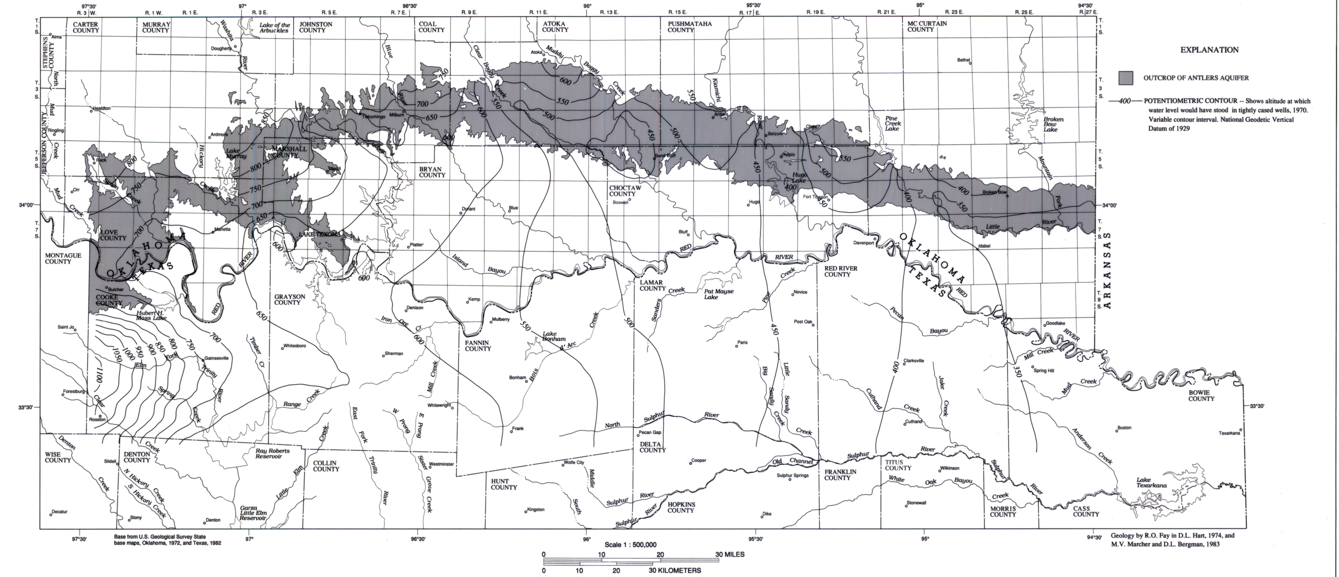
A. MAP SHOWING COMPUTED POTENTIOMETRIC SURFACE FOR THE STEADY-STATE SIMULATION OF 1970 HEAD DISTRIBUTION, ANTLERS AQUIFER
