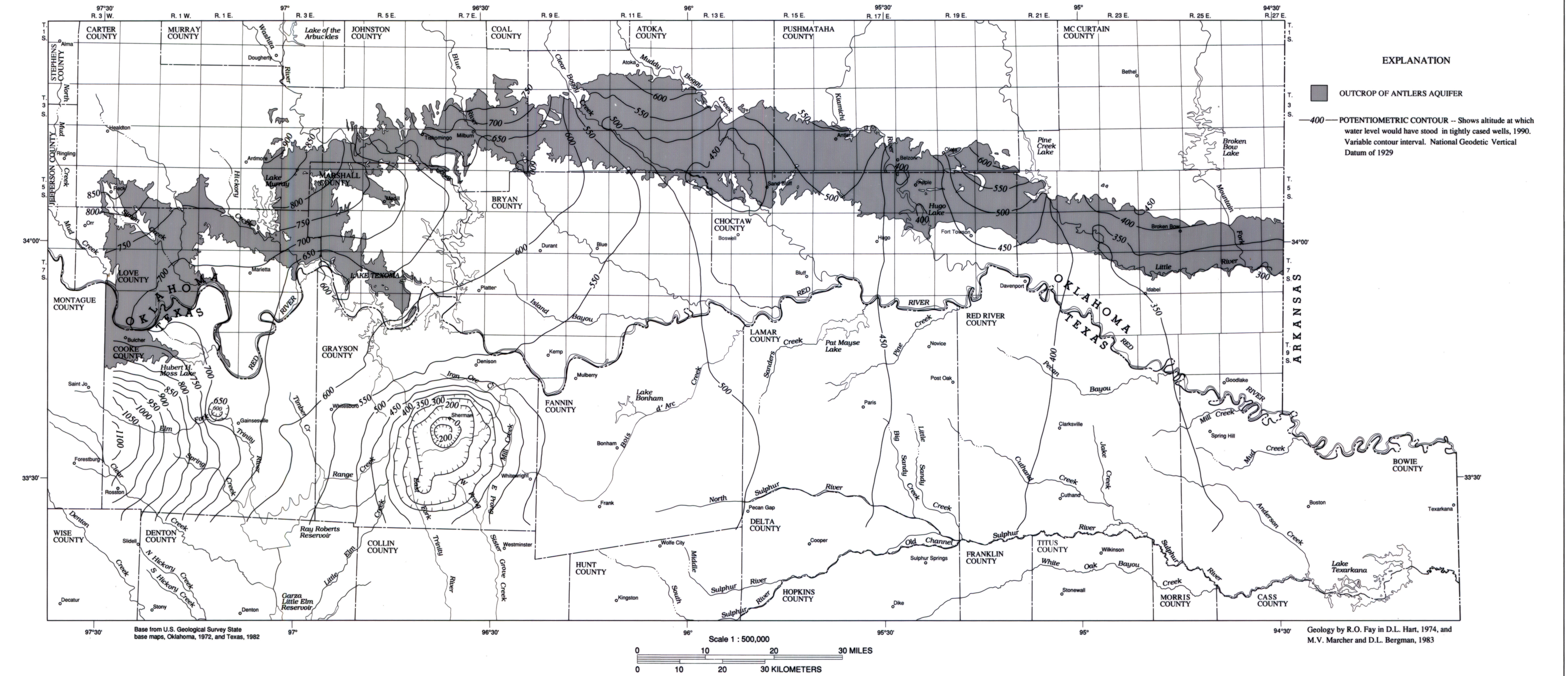
B. MAP SHOWING POTENTIOMETRIC SURFACE IN THE ANTLERS AQUIFER, 1990
