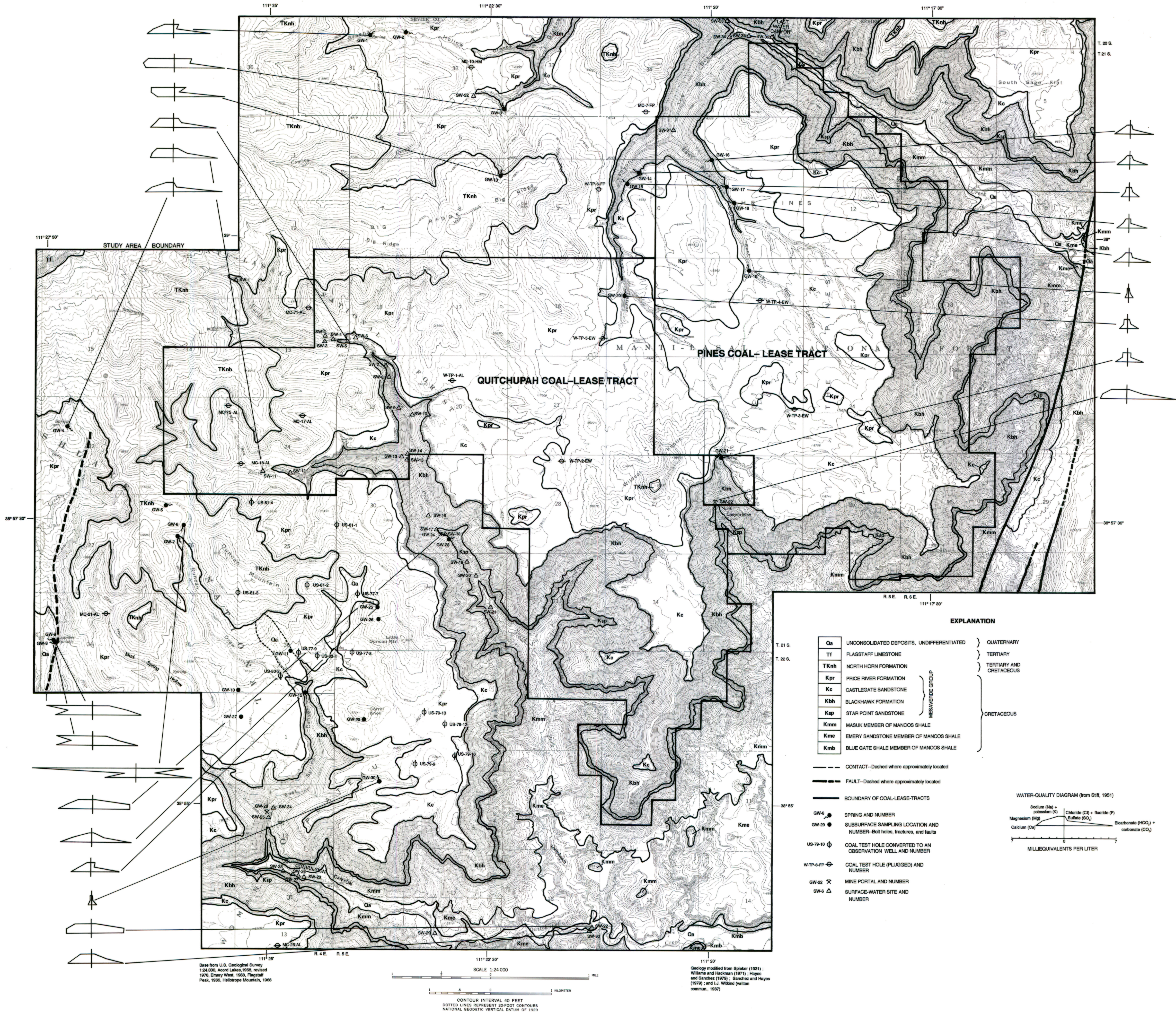
MAP SHOWING GEOLOGY, WATER-QUALITY DIAGRAMS, AND LOCATION OF HYDROLOGIC-DATA-COLLECTION SITES IN THE QUITCHUPAH AND PINES STUDY AREA, UTAH
