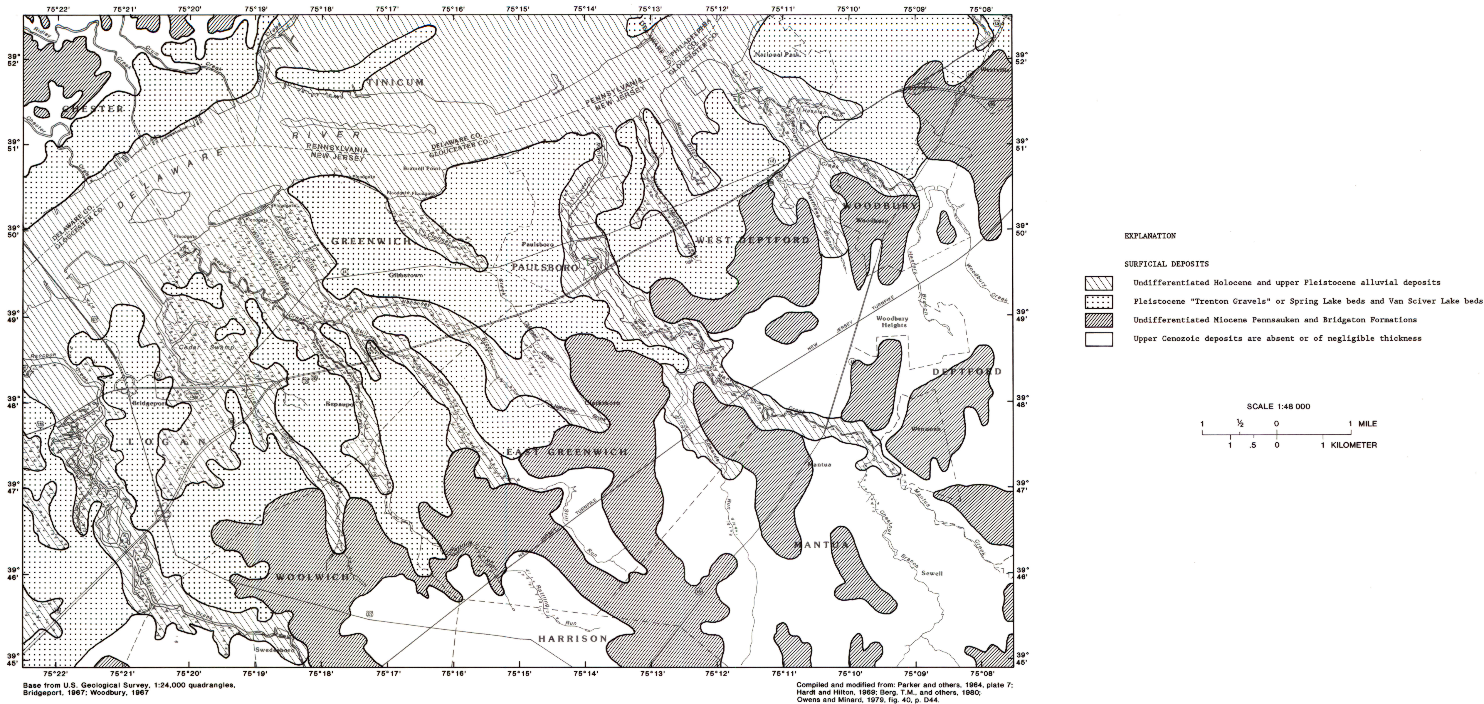
3a.--UPPER CENOZOIC DEPOSITS IN THE REGION OF GREENWICH TOWNSHIP, GLOUCESTER COUNTY, NEW JERSEY
