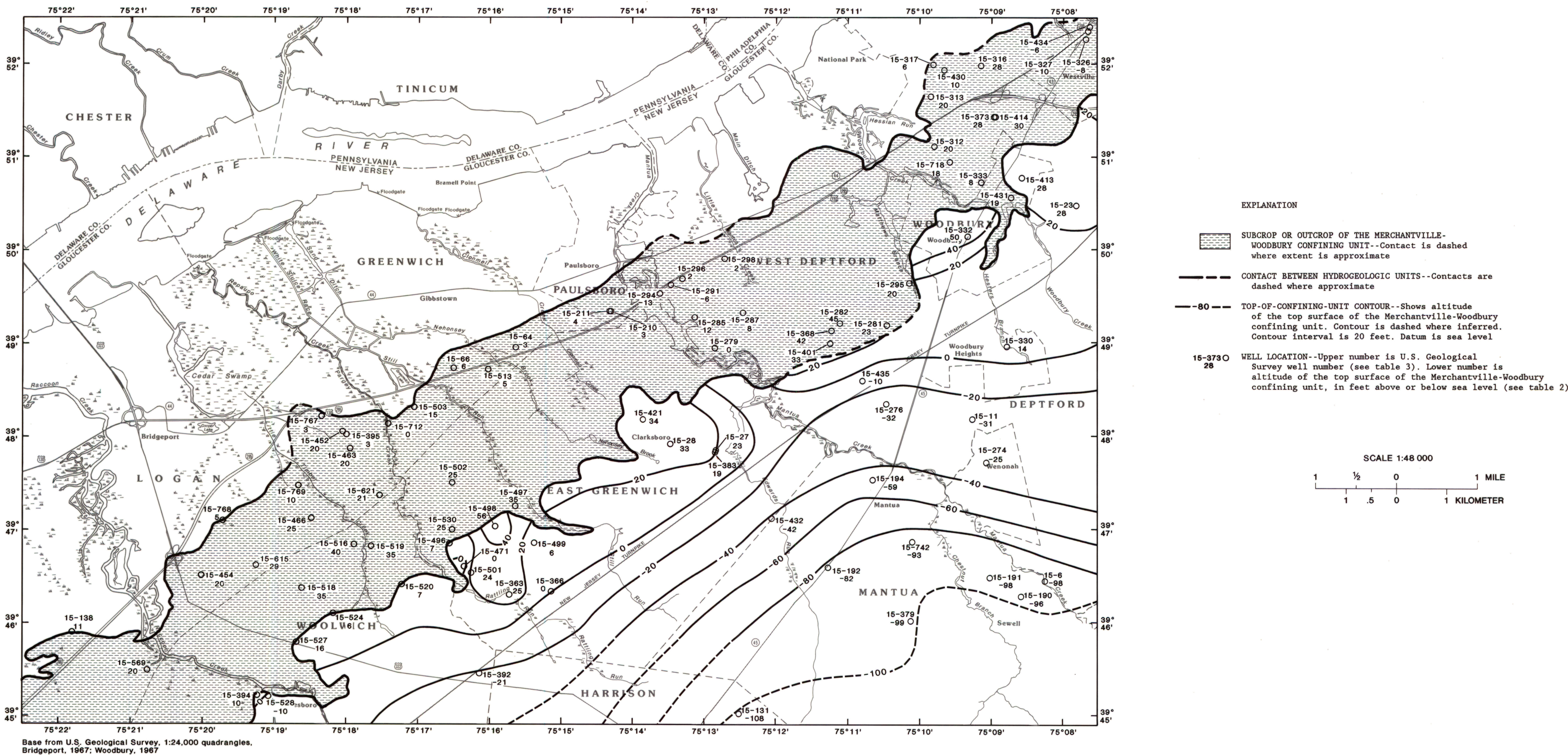
3b.--ALTITUDE OF THE TOP OF THE MERCHANTVILLE-WOODBURY CONFINING UNIT IN THE REGION OF GREENWICH TOWNSHIP, GLOUCESTER COUNTY, NEW JERSEY.
