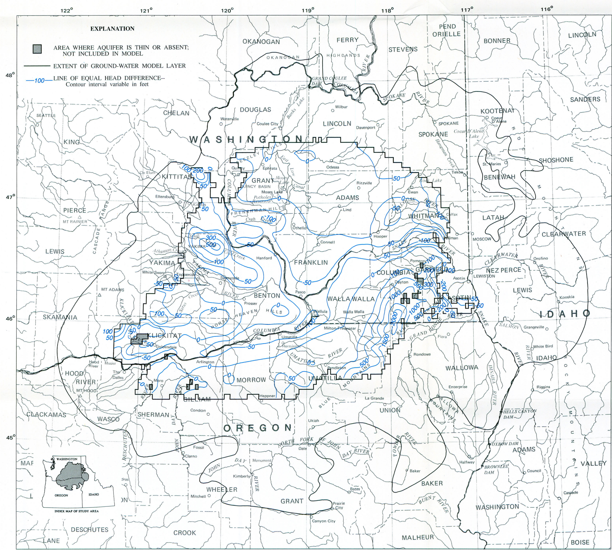
d. From the upper Grande Ronde to the lower Grande Ronde.
