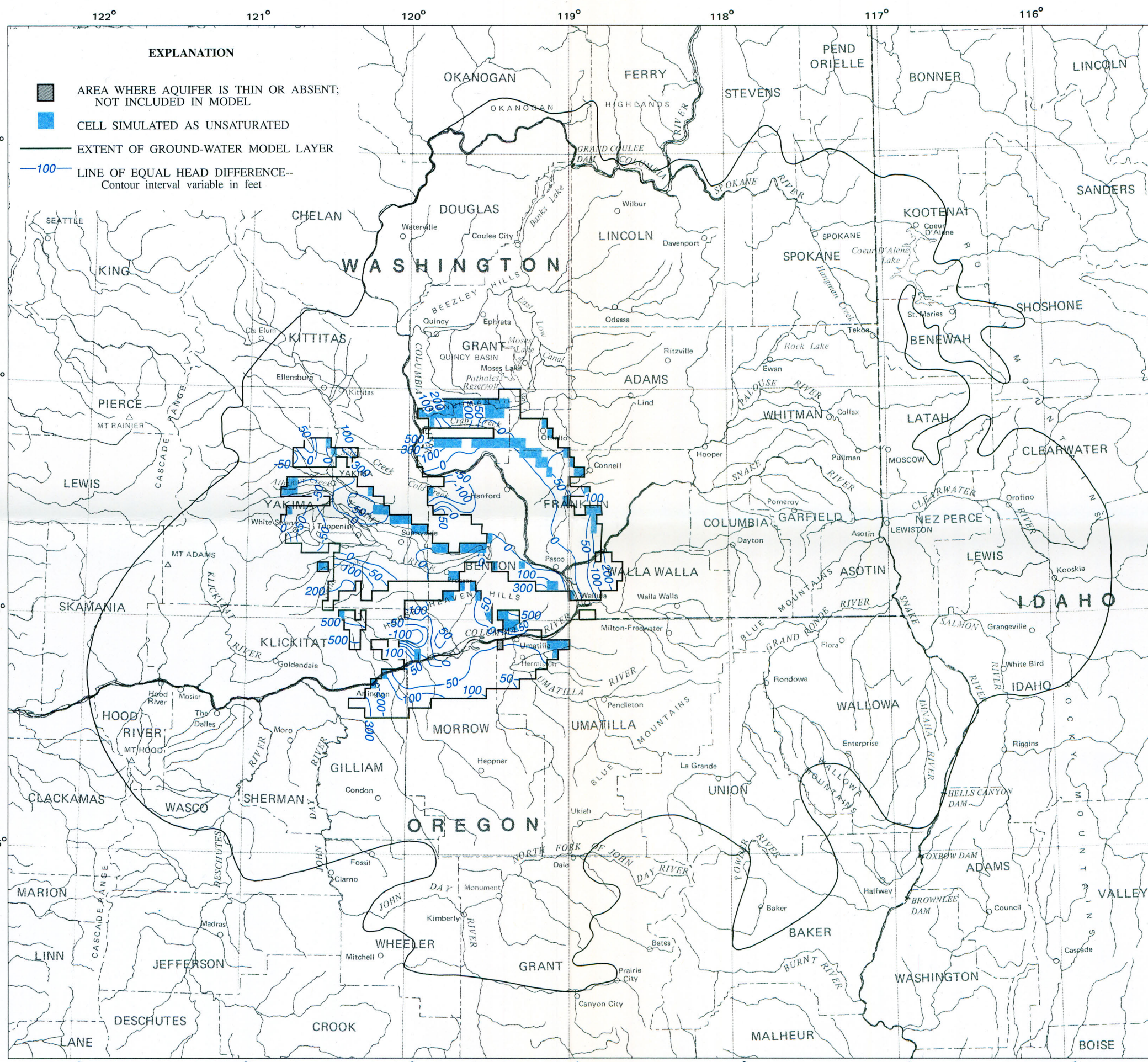
b. From the Saddle Mountains unit to the underlying unit.
