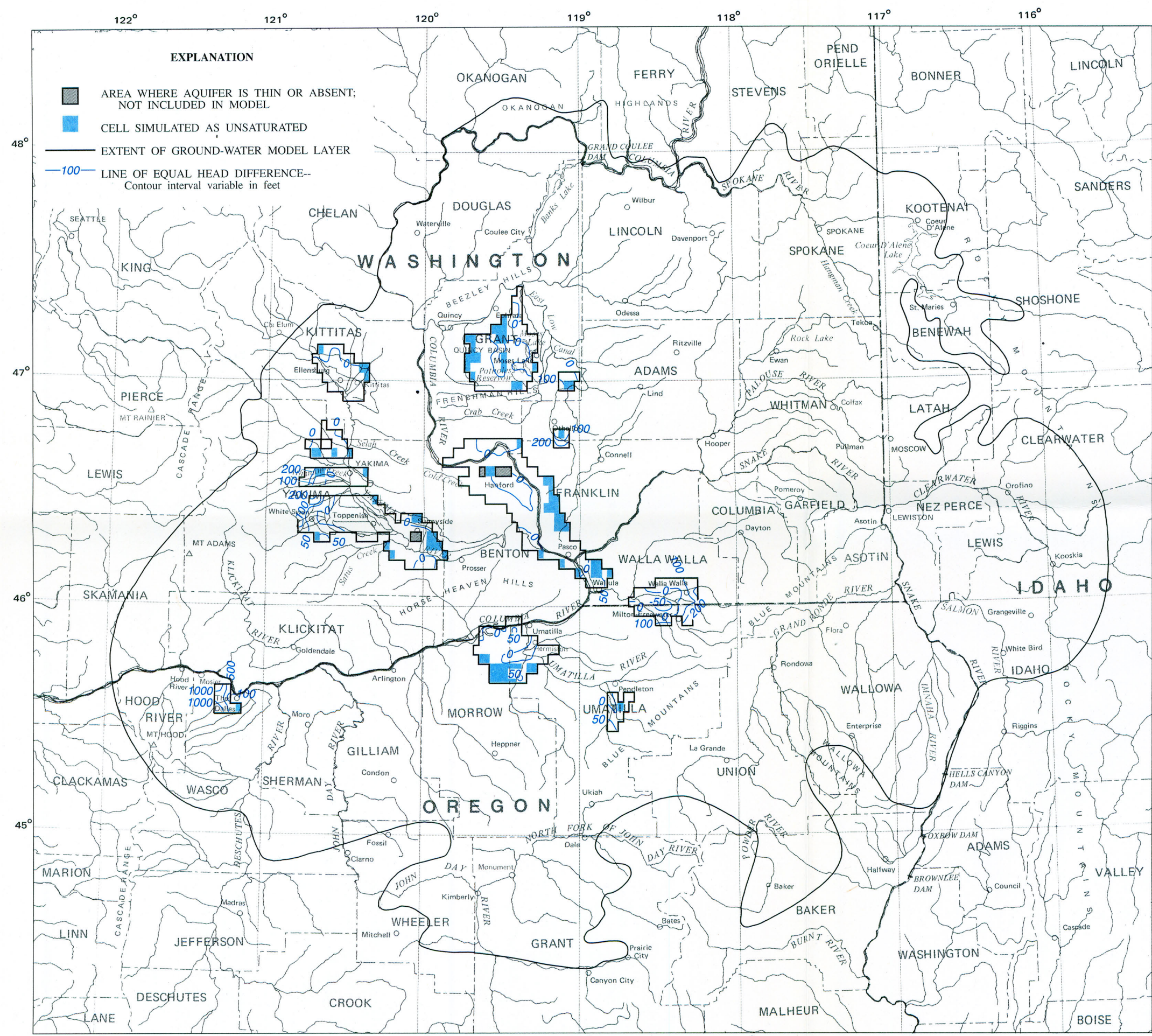
a. From the overburden aquifer to the underlying unit.
