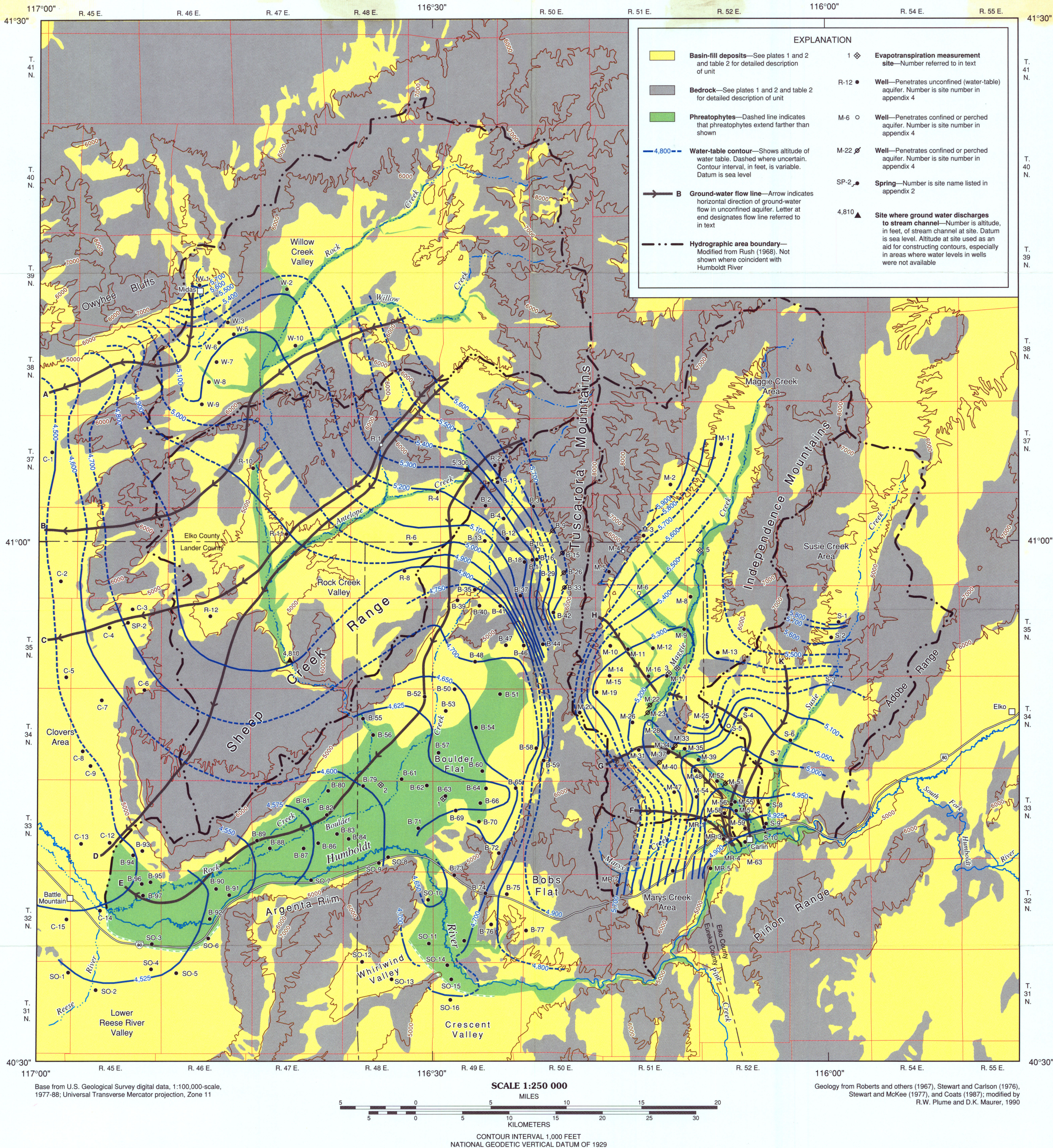
MAP SHOWING ALTITUDE OF UNCONFINED GROUND-WATER LEVELS, 1990-91, AND DISTRIBUTION OF PHREATOPHYTES, CARLIN TREND AREA, NORTH-CENTRAL NEVADA
