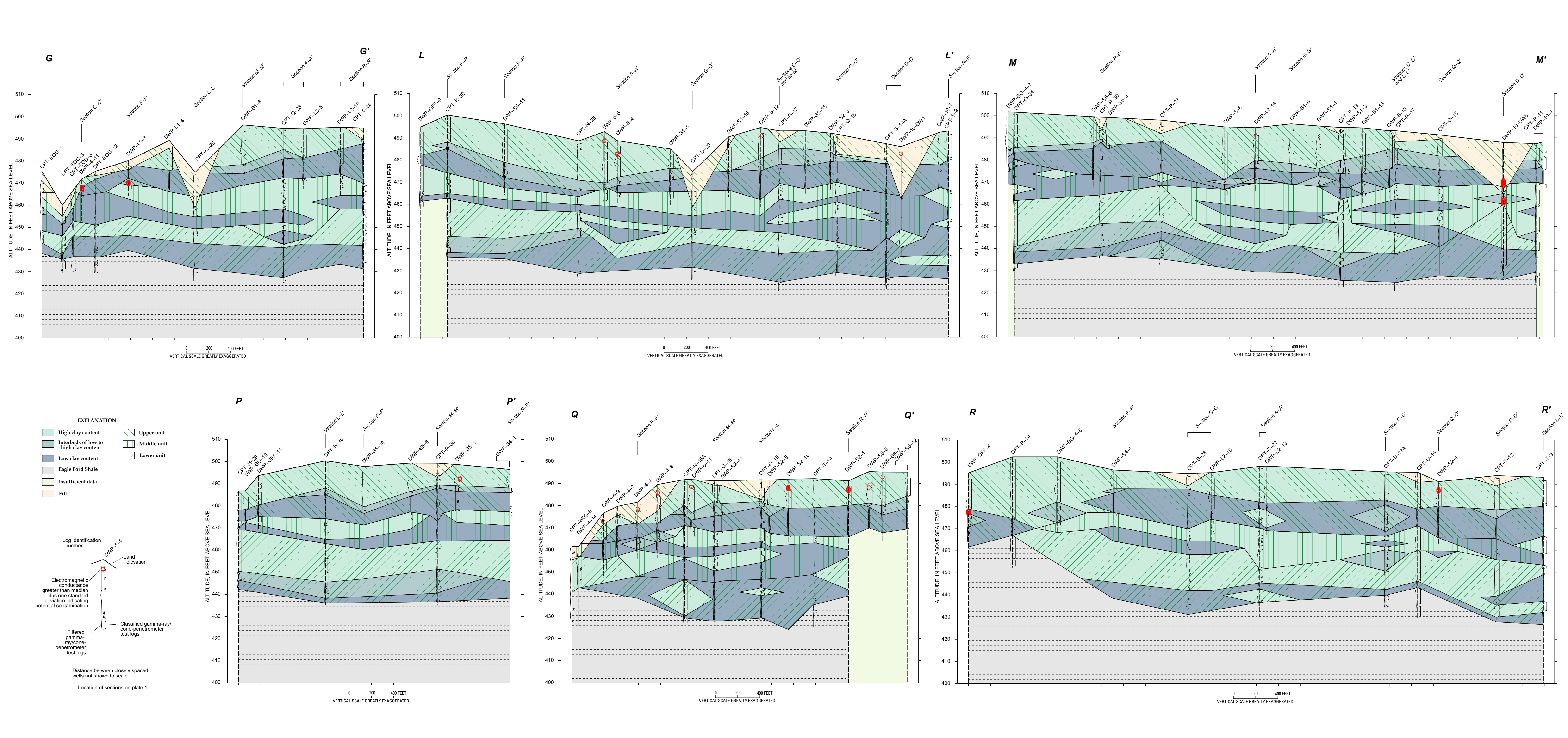
MAP SHOWING LITHOLOGIC SECTIONS G-G', L-L', M-M', P-P', Q-Q', AND R-R' AT NAVAL WEAPONS INDUSTRIAL RESERVE PLANT, DALLAS, TEXAS By Roberto Anaya, Christopher L. Braun, and Eve L. Kuniansky 2000
