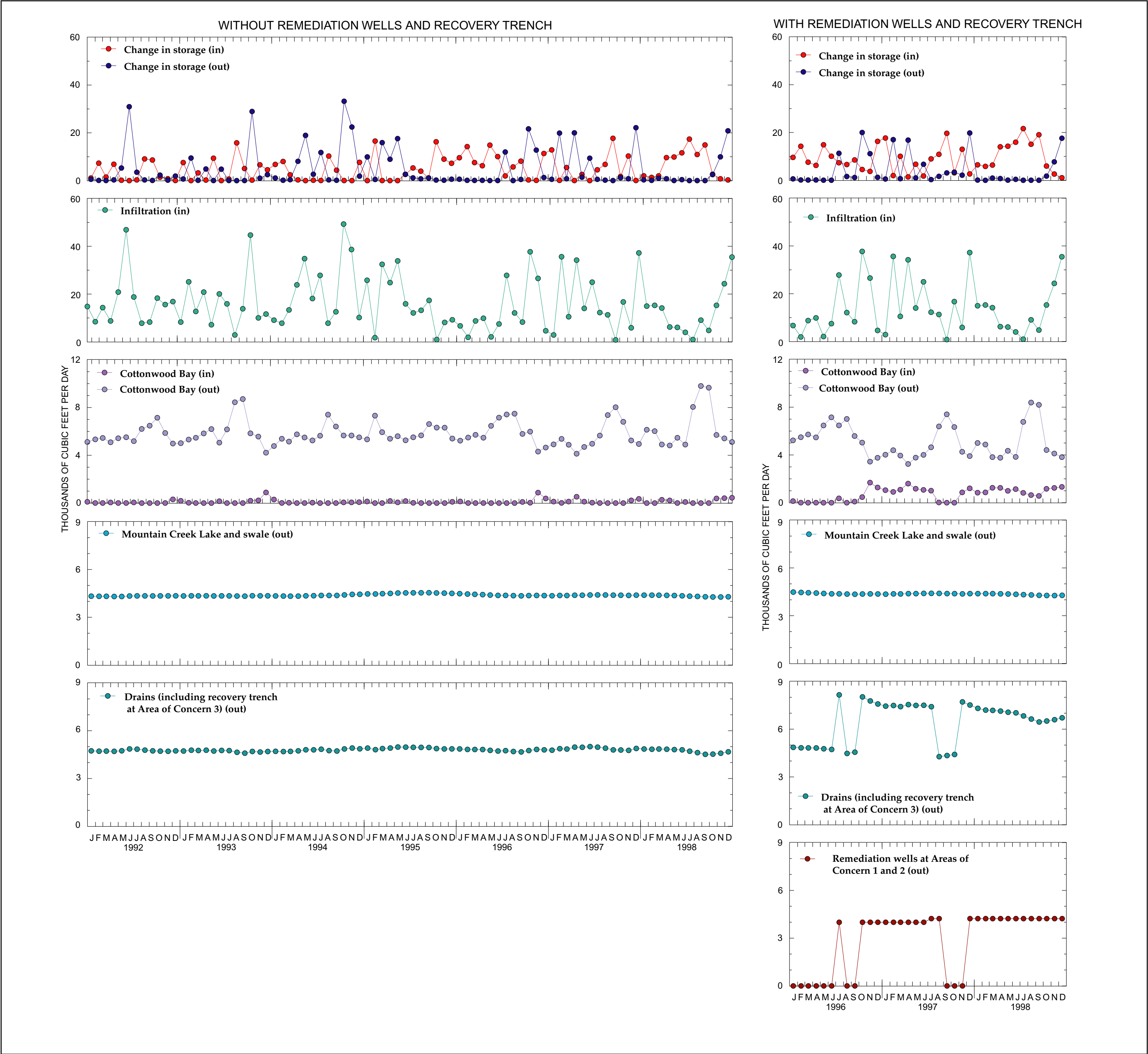
HYDROGRAPHS SHOWING SIMULATED RATES OF RECHARGE TO (IN) AND DISCHARGE FROM (OUT) THE SHALLOW ALLUVIAL AQUIFER UNDERLYING THE STUDY AREA, WITHOUT AND WITH REMEDIATION WELLS AND RECOVERY TRENCH, 1992-98
