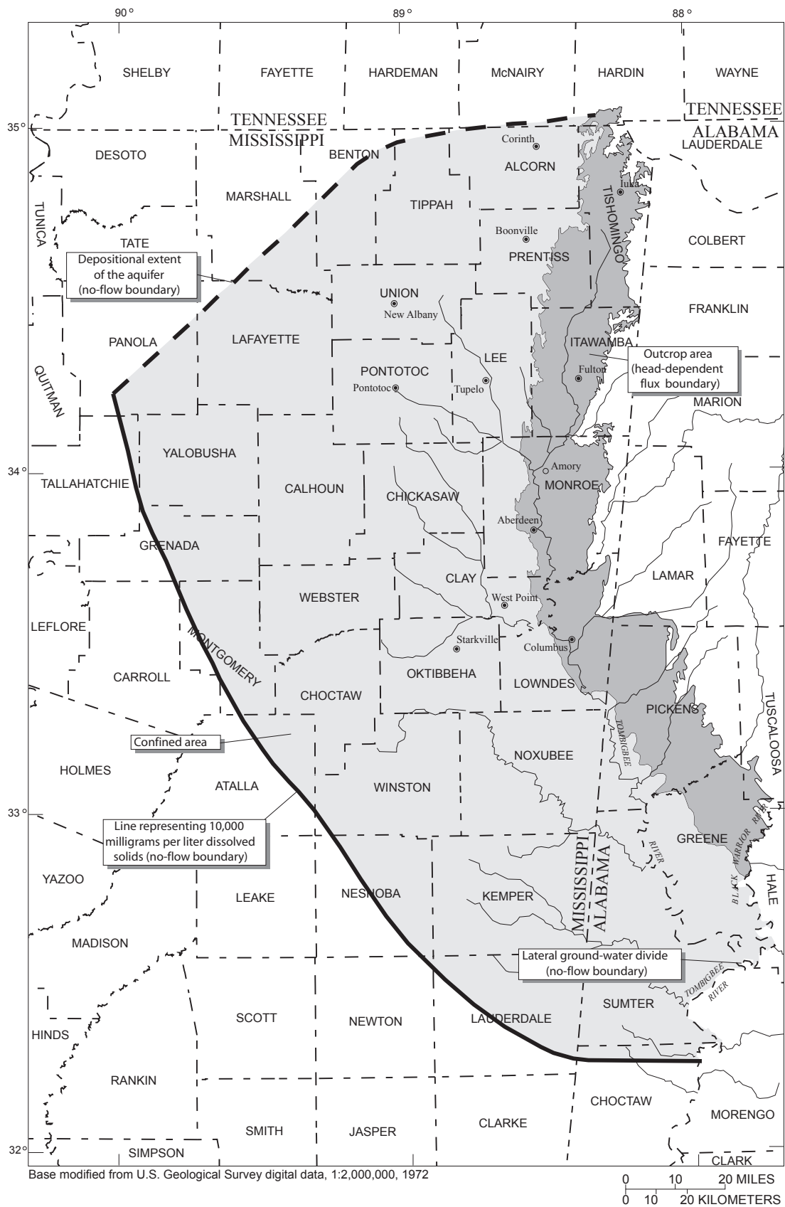
Figure 4. The extent of the Eutaw-McShan aquifer, Mississippi and Alabama.
