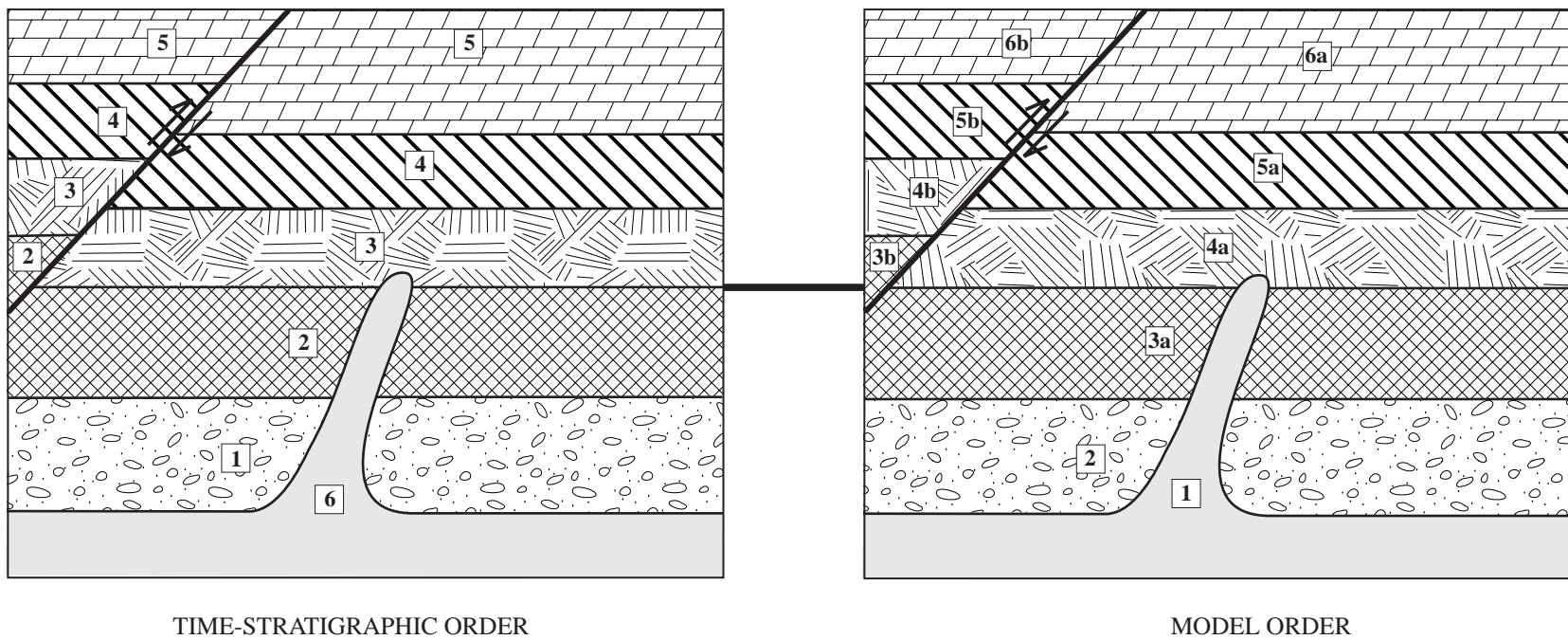
Figure 8. Time-stratigraphic and model order of geologic events (from D'Agnesi and others, 1997).
