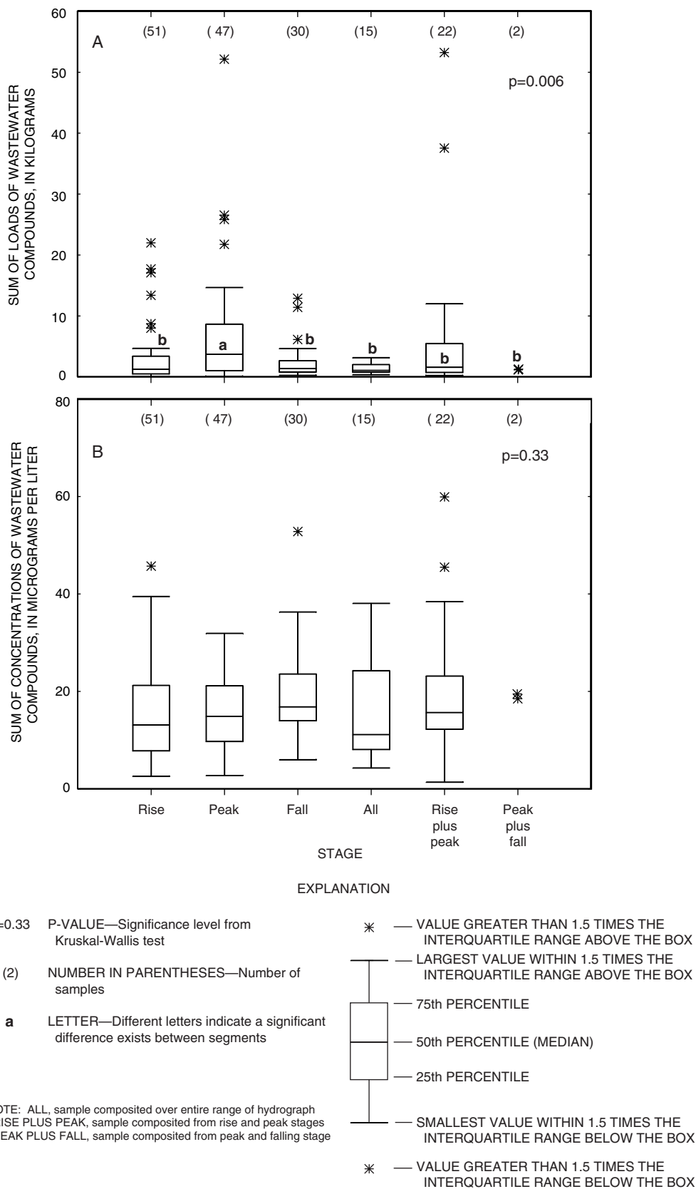
Figure 11. Sum of loads (A) and sum of concentrations (B) for wastewater indicator compounds in storm hydrograph segments.
