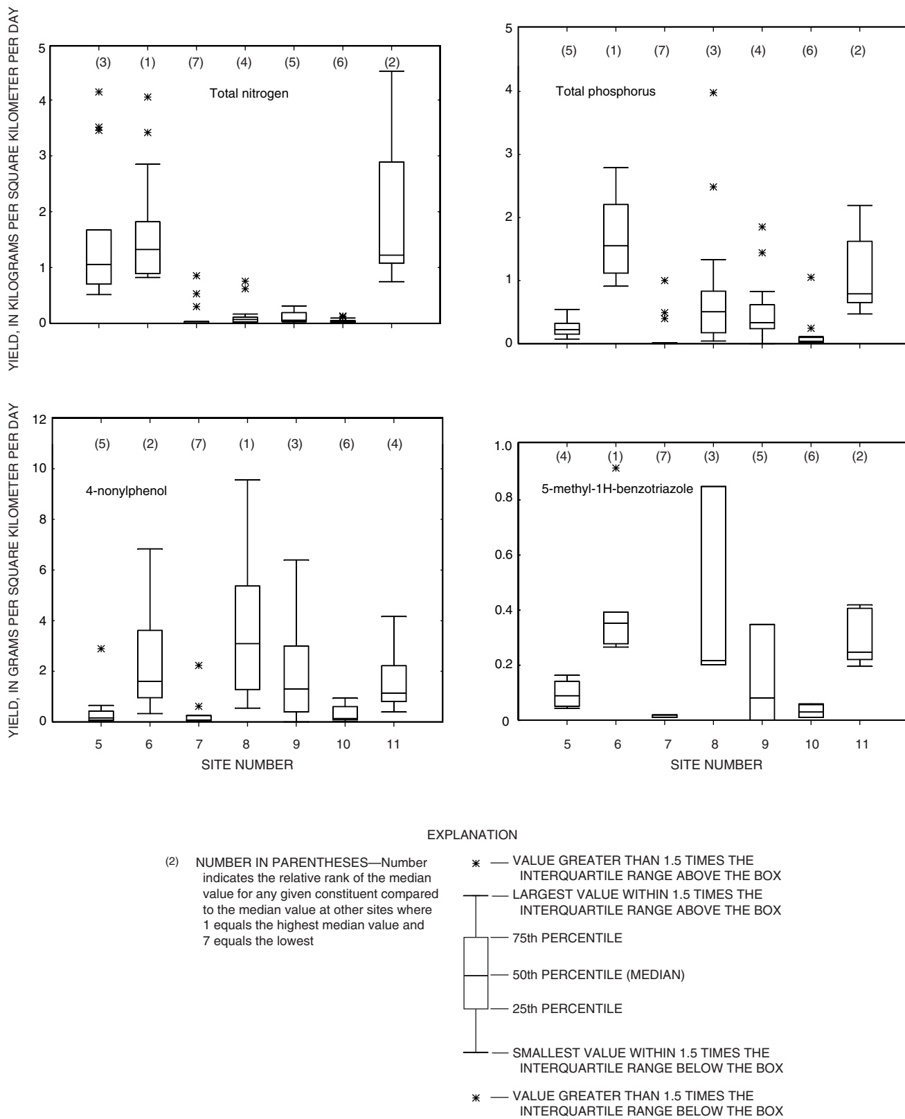
Figure 12. Yield of selected constituents in base-flow samples.
