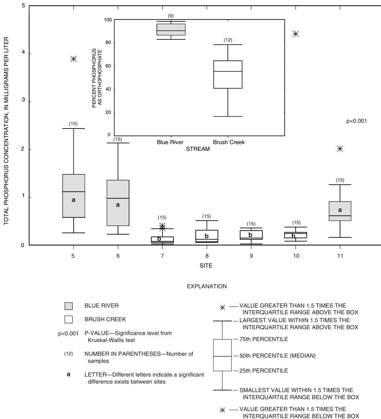
Figure 6. Total phosphorus concentration by site and the percentage of the total phosphorus that is ortho-phosphate by stream (inset) in base-flow samples.
