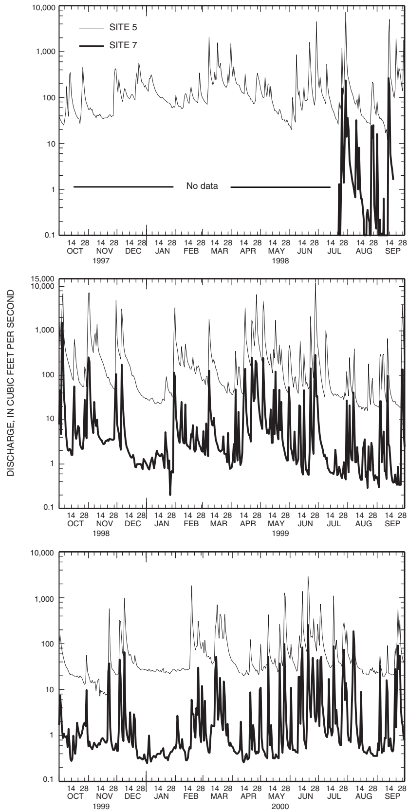
Figure 2. Mean daily discharge for Blue River near Kansas City (site 5) and Brush Creek at Ward Parkway (site 7) from October 1997 through September 2000.
