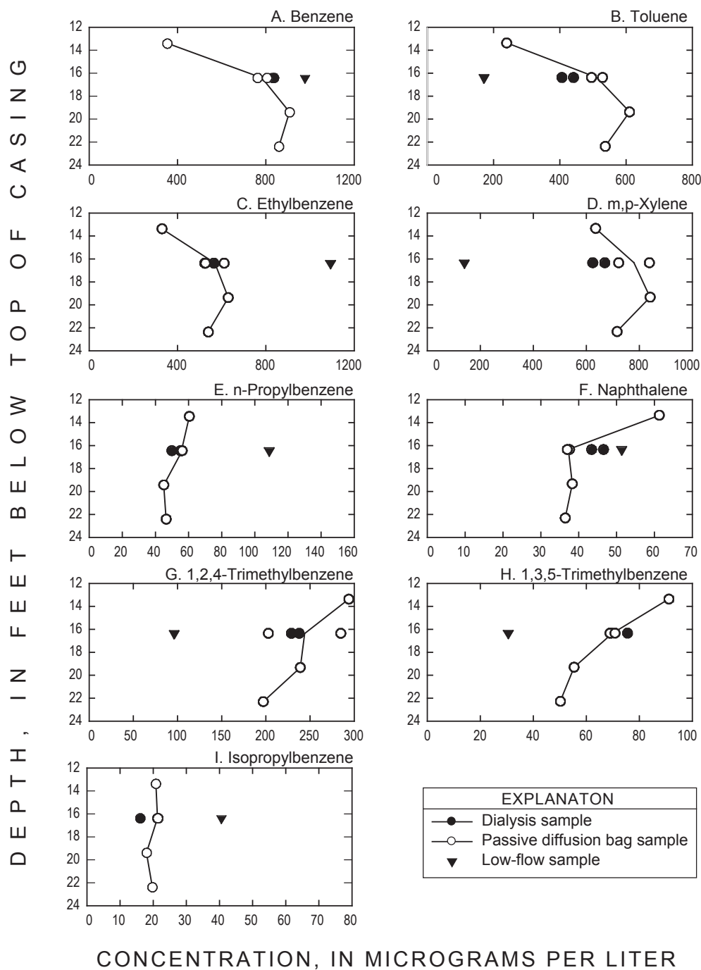
Figure 6. Vertical distributions of volatile organic compounds in dialysis and low-flow samples from well SS01 MW-12, Hickam Air Force Base, Hawaii, July 2001.
