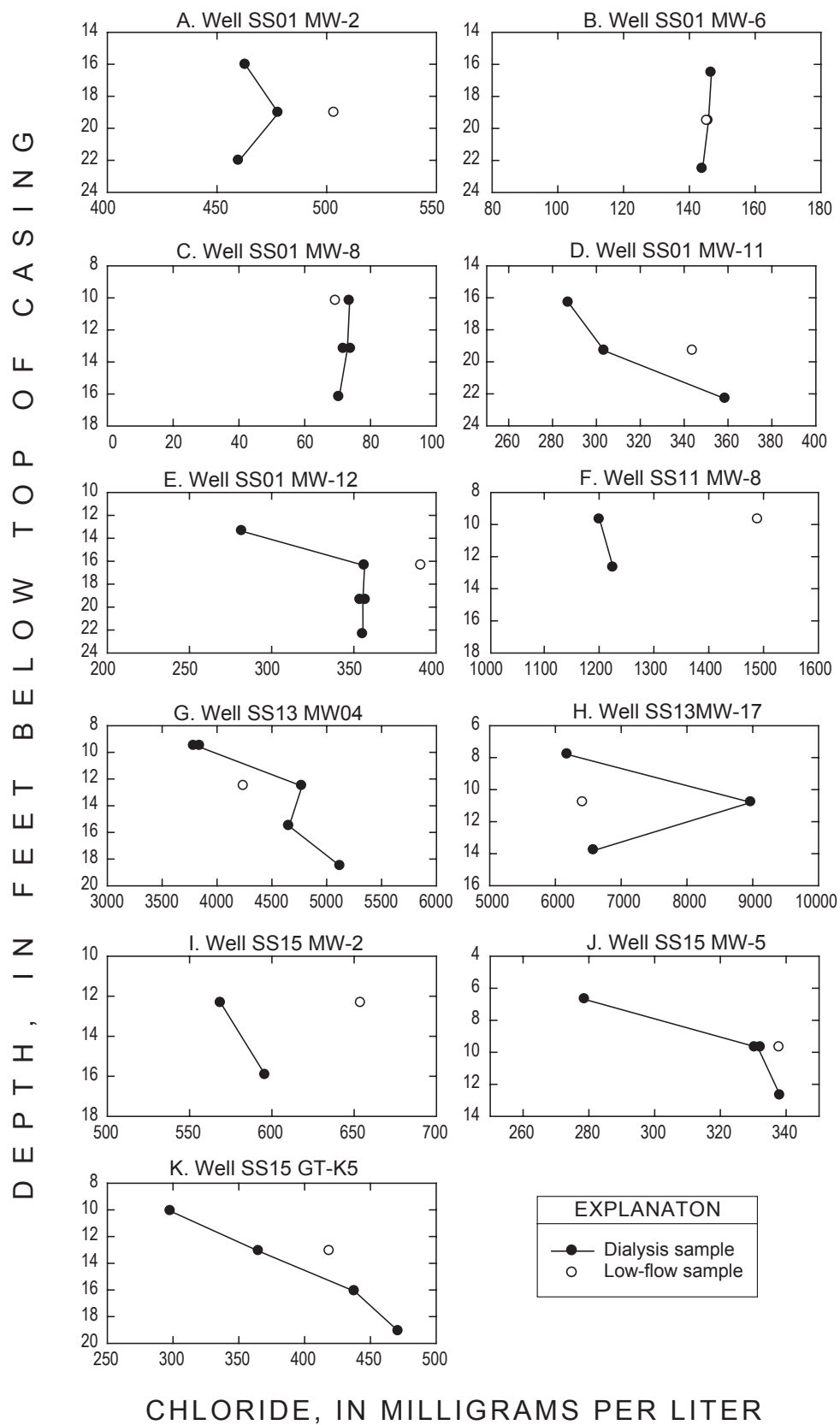
Figure 4. Vertical distribution of chloride in dialysis and low-flow samples from wells at Hickam Air Force Base, Hawaii, July 2001.
