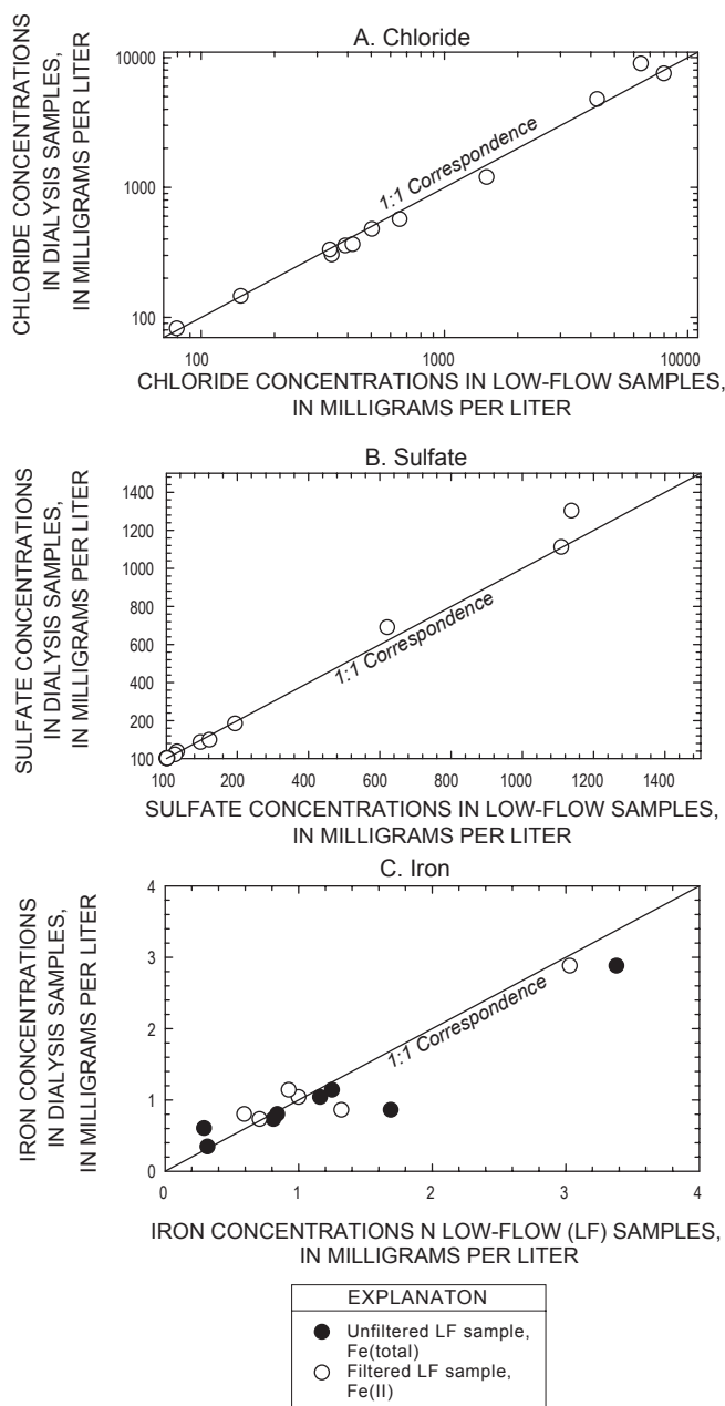
Figure 3. Comparison of chloride, sulfate, and iron concentrations in low-flow samples to concentrations in dialysis samples at the same depth, Hickam Air Force Base, Hawaii, July 2001.
