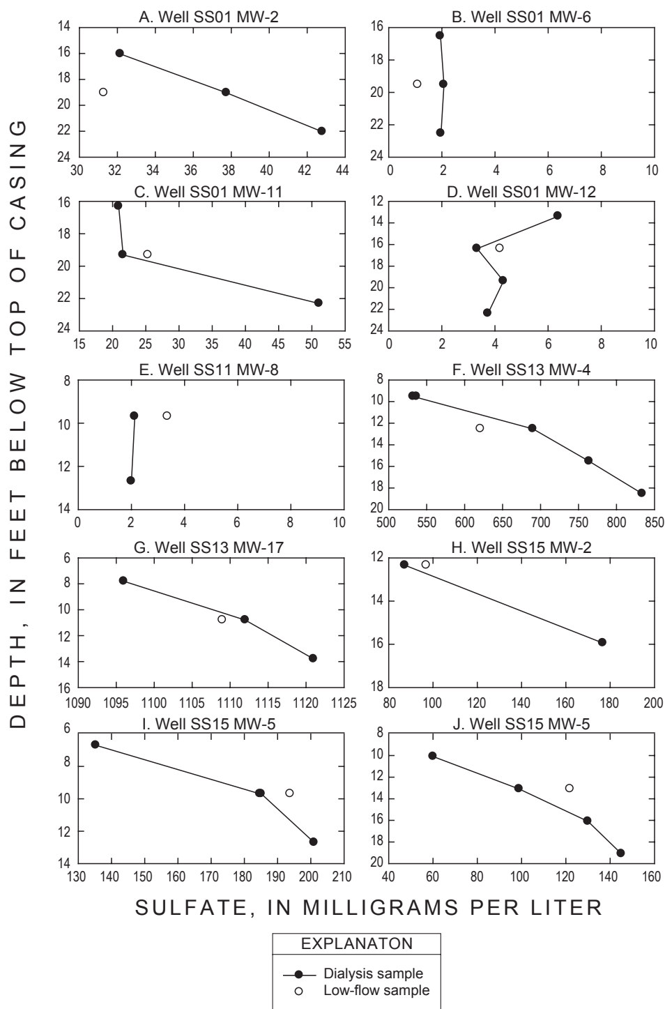
Figure 5. Vertical distribution of sulfate in dialysis and low-flow samples from wells at Hickam Air Force Base, Hawaii, July 2001.
