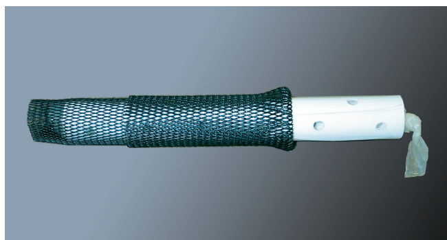
Figure 2. Dialysis bag on perforated pipe with the outer low-density polyethylene mesh pulled partway back.
