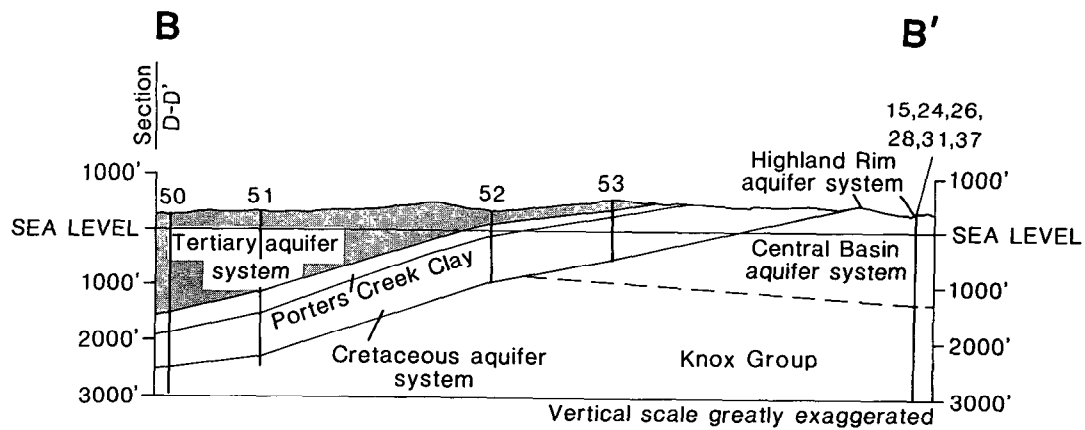
Figure 4.-- Geohydrologic section showing water quality in the Tertiary aquifer system along line B-B'.
