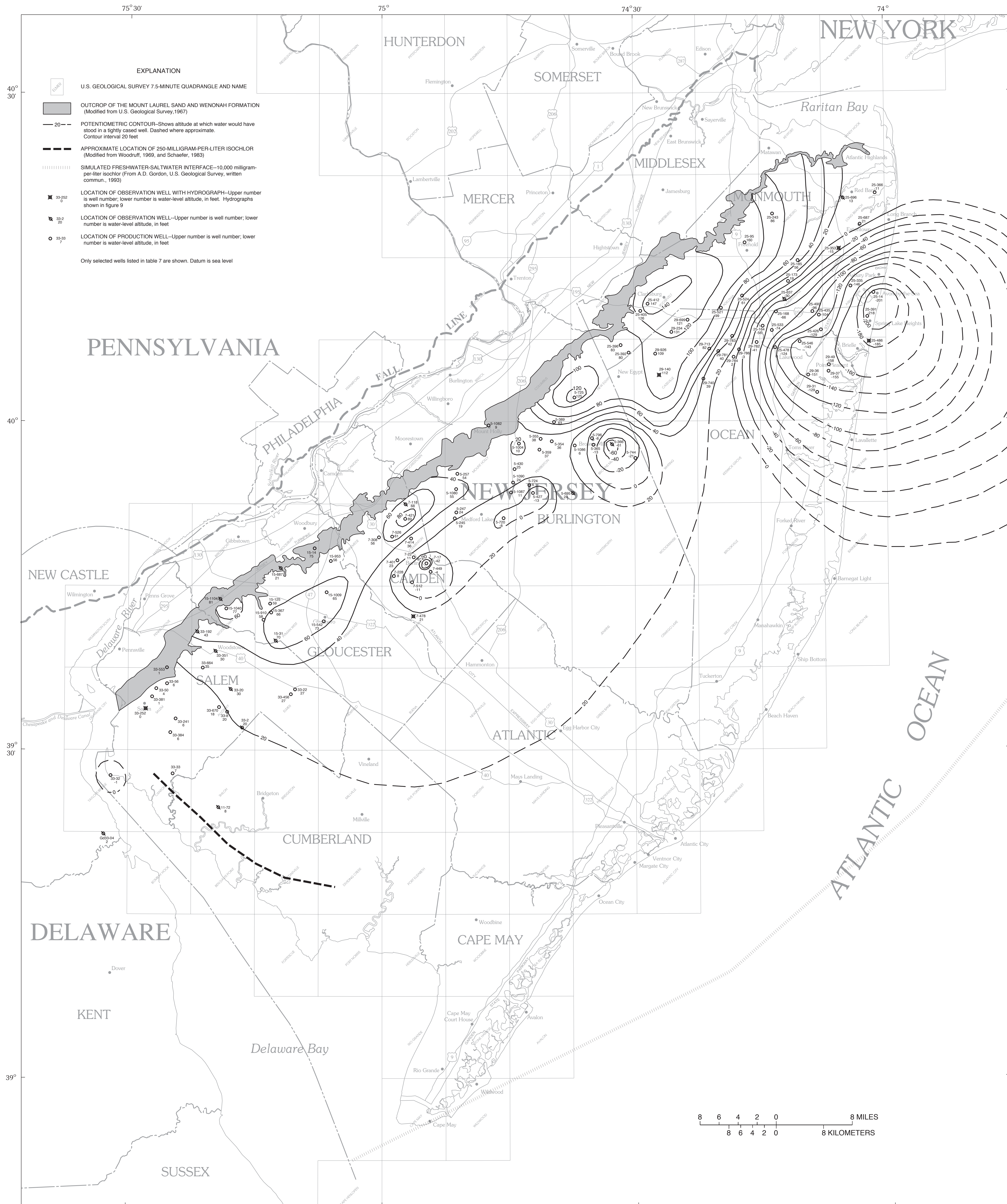
POTENTIOMETRIC SURFACE OF THE WENONAH-MOUNT LAUREL AQUIFER, 1988
