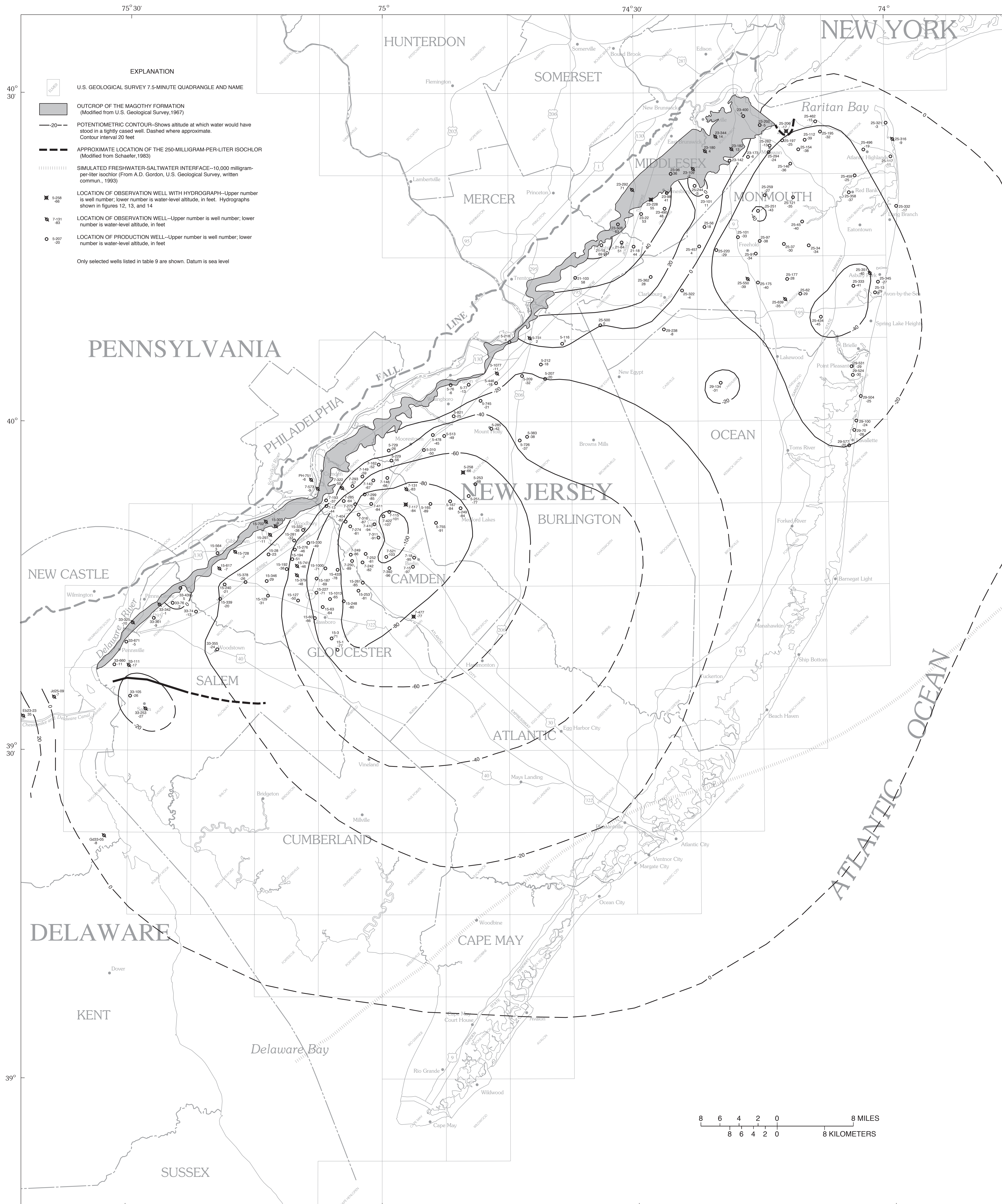
POTENTIOMETRIC SURFACE OF THE UPPER AQUIFER OF THE POTOMAC-RARITAN-MAGOTHY AQUIFER SYSTEM, 1988
