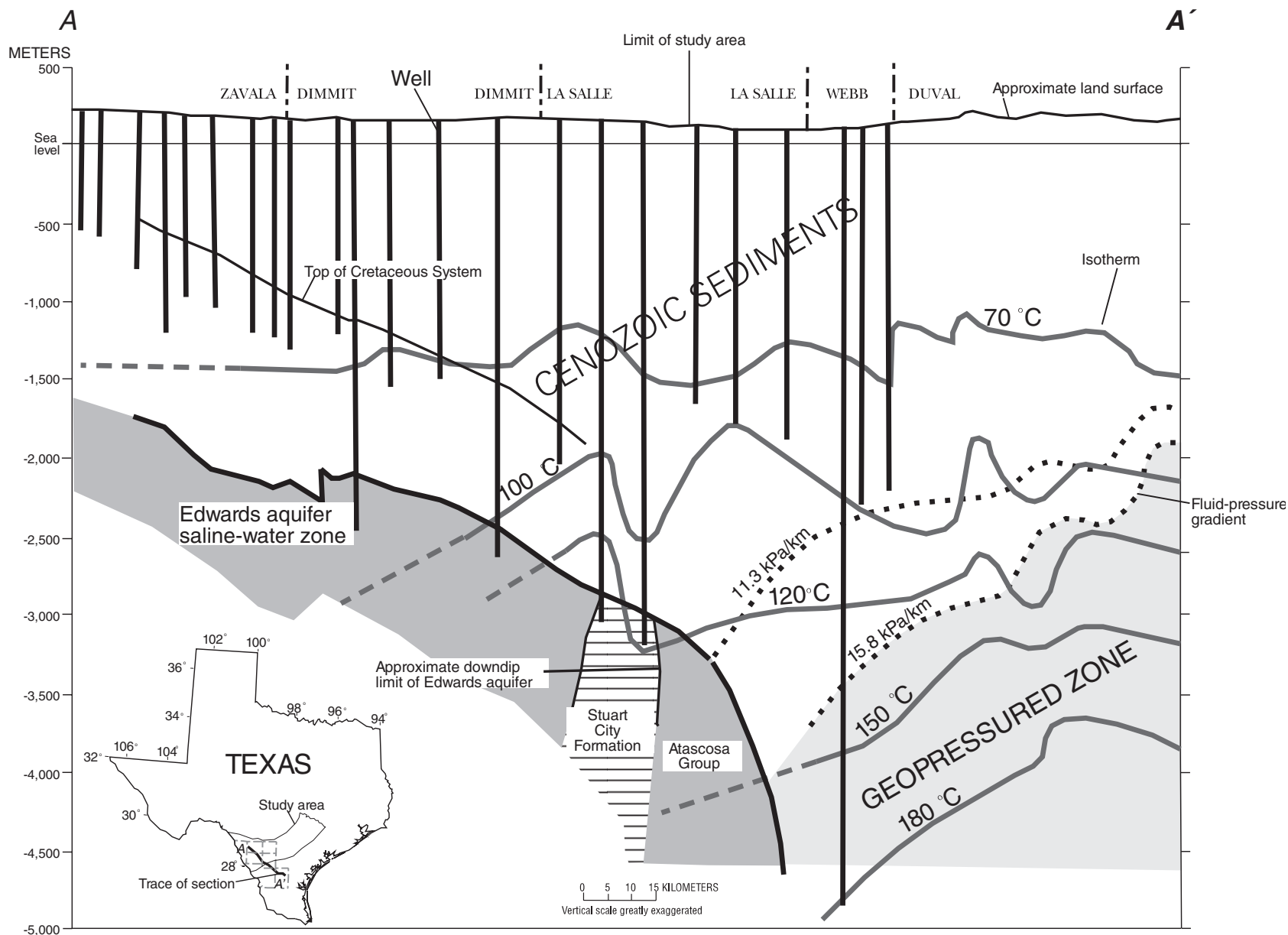
Figure 5. Generalized hydrogeologic section showing the relation between the Edwards aquifer and the geopressured zone in the subsurface of the Texas Gulf Coast.
