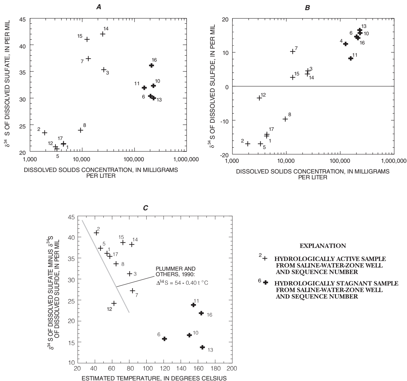
Figure 12. Relations between (A) del sulfur-34 ( \delta^{34}\text{S} ) of dissolved sulfate and dissolved solids concentration, (B) \delta^{34}\text{S} of dissolved sulfide and dissolved solids concentration, and (C) \delta^{34}\text{S} of dissolved sulfate minus \delta^{34}\text{S} of dissolved sulfide and estimated temperature in ground-water samples from the Edwards aquifer saline-water zone, south-central Texas.
