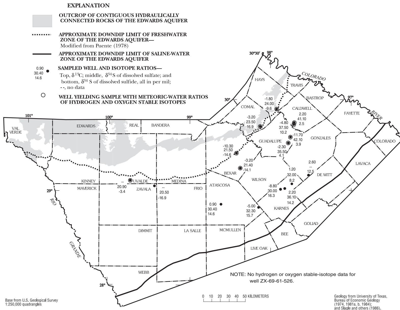
Figure 13. Distribution of del carbon-13 ( \delta^{13}\text{C} ) of dissolved inorganic carbon and del sulfur-34 ( \delta^{34}\text{S} ) of dissolved sulfate and sulfide in ground-water samples, and location of wells that produce water with meteoric del deuterium ( \delta\text{D} ) and del oxygen-18 ( \delta^{18}\text{O} ) in the Edwards aquifer saline-water zone, south-central Texas.
