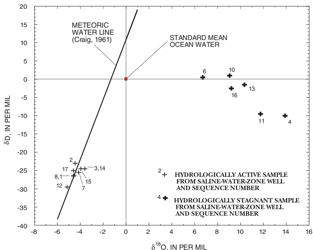
Figure 16. Relation between del deuterium ( \delta D ) and del oxygen-18 ( \delta^{18}O ) in ground-water samples from the Edwards aquifer saline-water-zone, south-central Texas.
