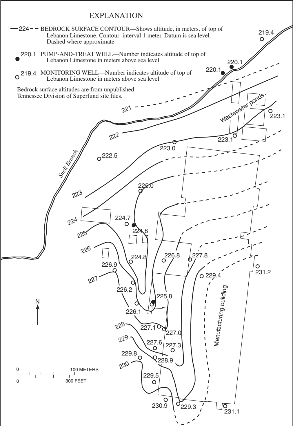
Figure 6. Bedrock surface at the study site.
