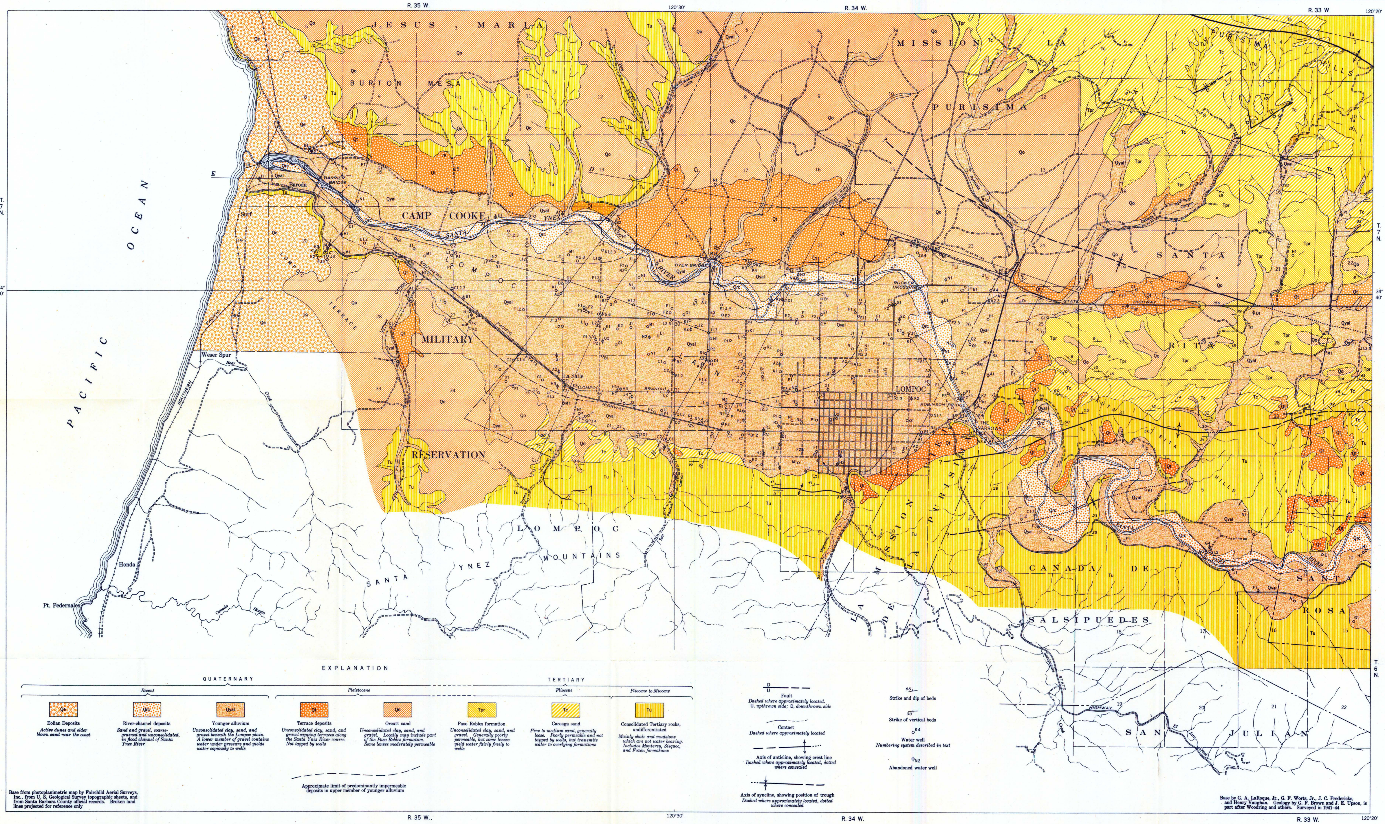
GEOLOGIC MAP OF THE WESTERN PART OF THE SANTA YNEZ RIVER BASIN
