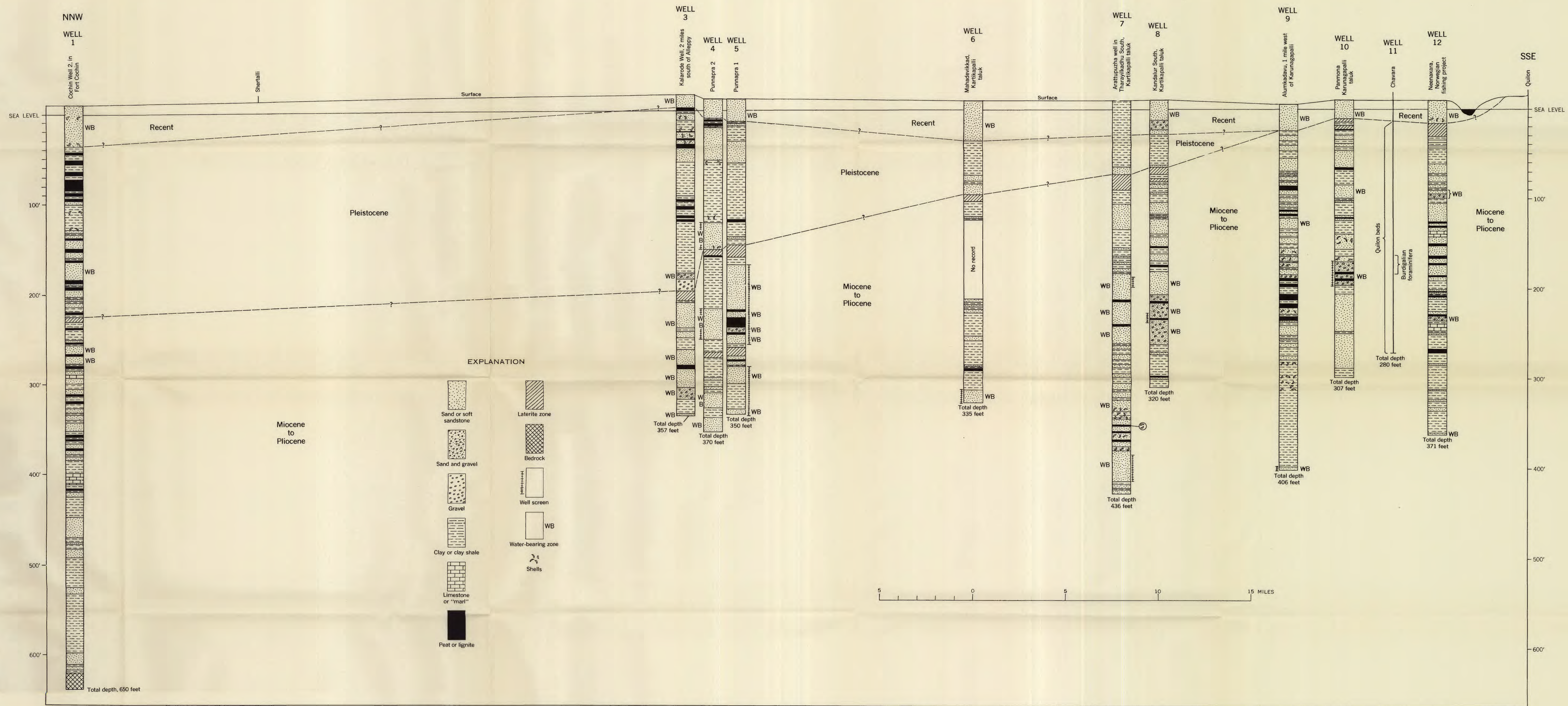
GEOLOGIC SECTION ALONG THE COAST OF KERALA FROM COCHIN TO QUILON, INDIA
