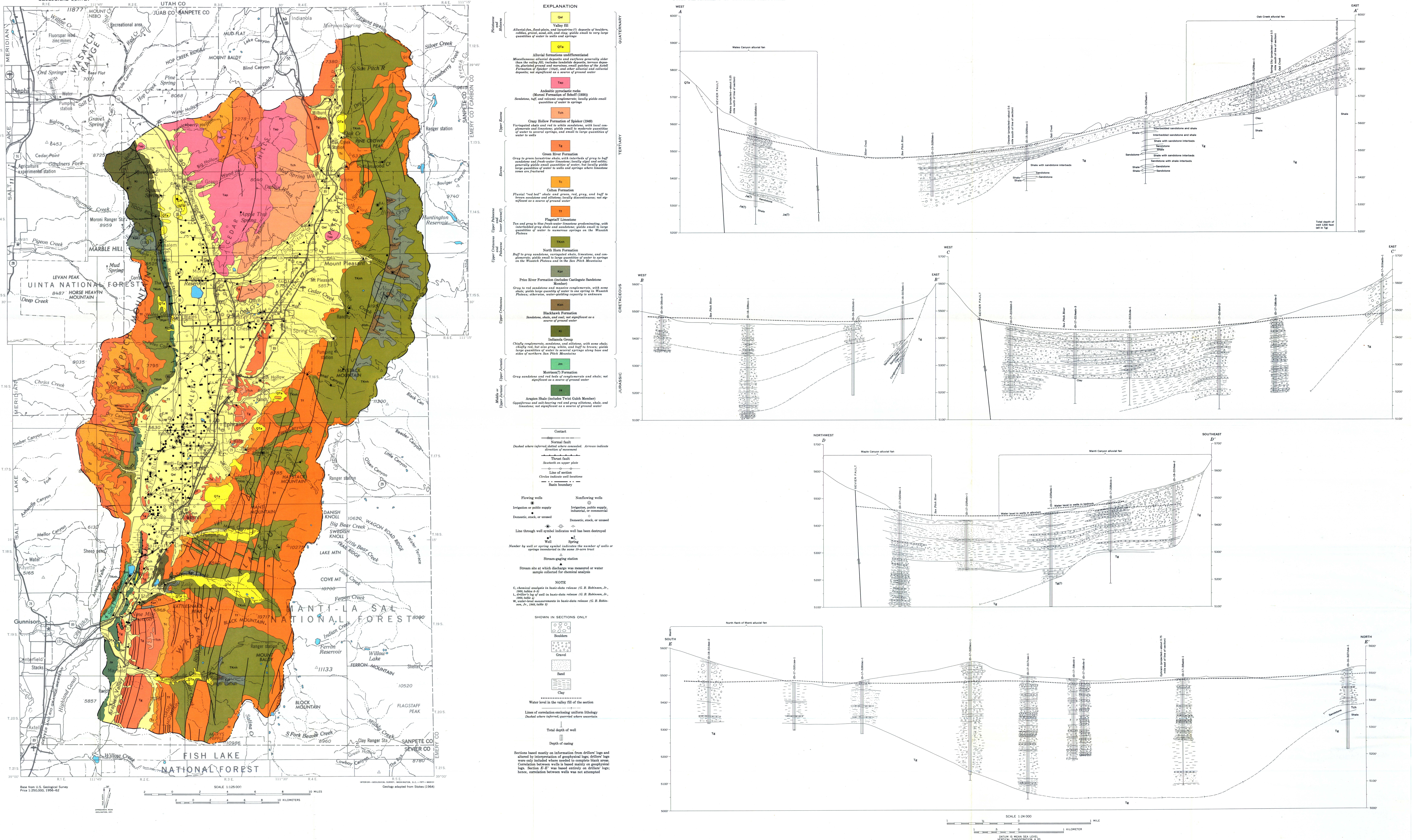
GENERALIZED GEOLOGIC MAP AND SECTIONS SHOWING LOCATION OF SELECTED HYDROLOGIC DATA SITES, SAN PITCH RIVER DRAINAGE BASIN, SANPETE COUNTY, UTAH
