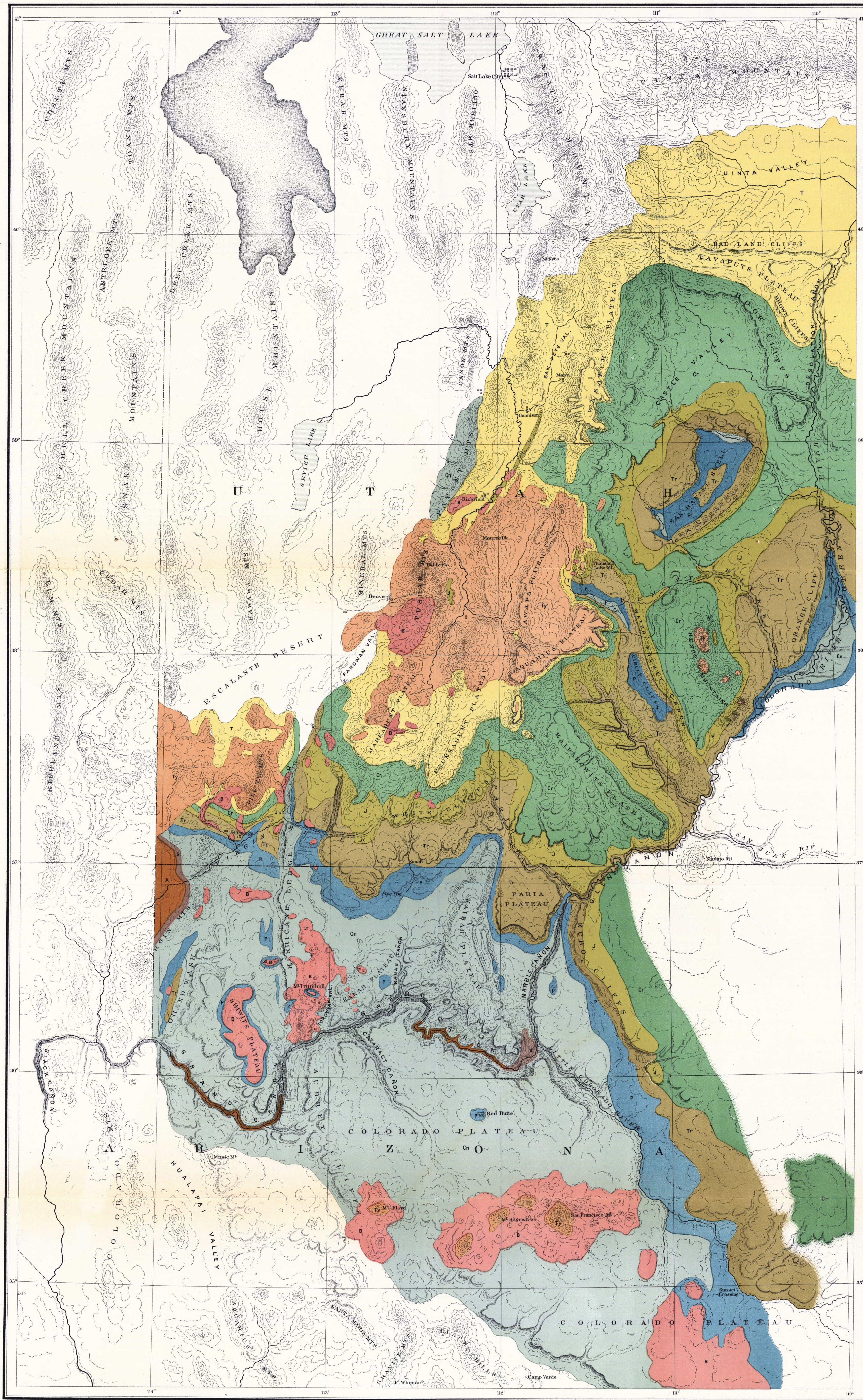
SKETCH MAP SHOWING THE DISTRIBUTION OF THE STRATA AND ERUPTIVE ROCKS IN THE WESTERN PART OF THE PLATEAU PROVINCE
