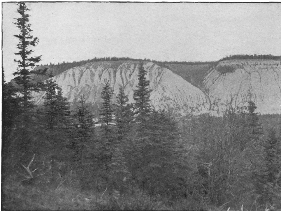
A. COPPER RIVER SILT BLUFFS ON KLUTENA.
