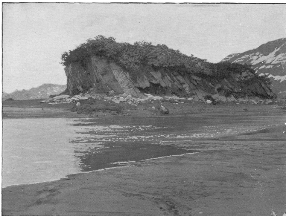
B. GIANT ROCK, SHOWING APLITE DIKES IN SLATE.
