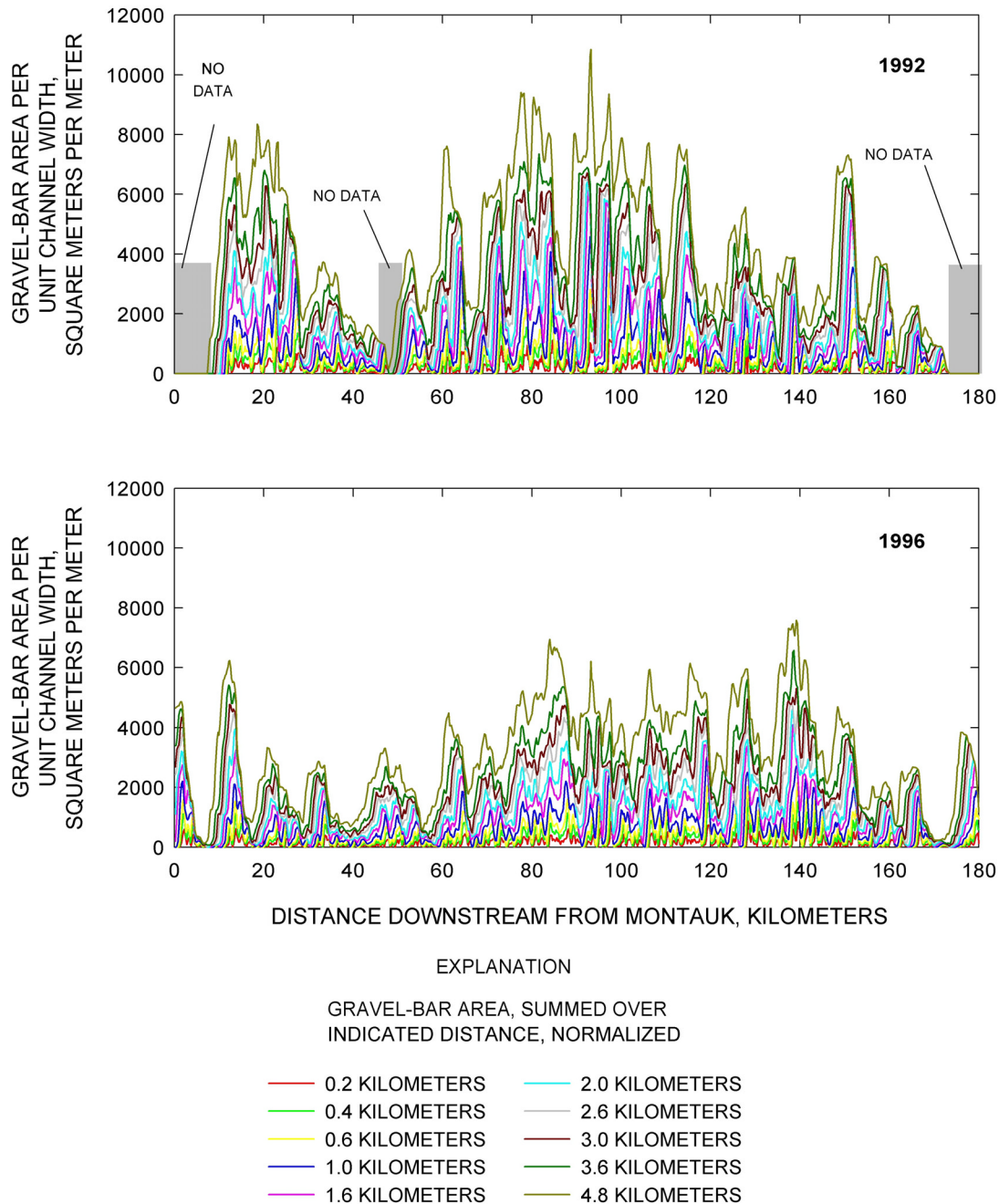
Plots of unit gravel-bar area summed over distances of 0.2 - 4.8 km downstream, plotted against distance downstream
