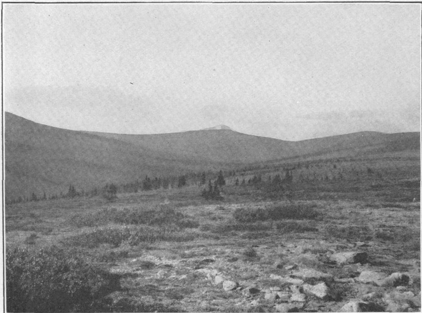
A. OPEN VALLEY, TRIBUTARY OF CHARLEY RIVER.
