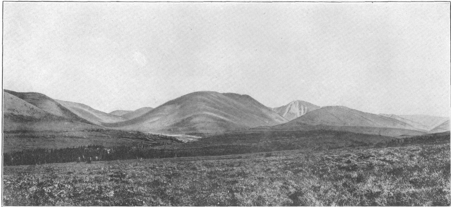
MORaine NEARLY FILLING MAIN VALLEY FROM SMALL VALLEY HEADING IN PEAK IN BACKGROUND.
