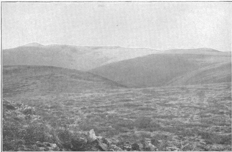
A. SCHIST RIDGE BETWEEN NORTH FORK OF BIRCH CREEK AND CROOKED CREEK.
