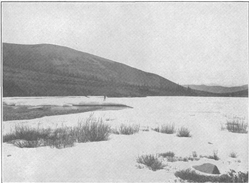
A. ICE-FILLED STREAM FLAT, GOODPASTURE RIVER.
