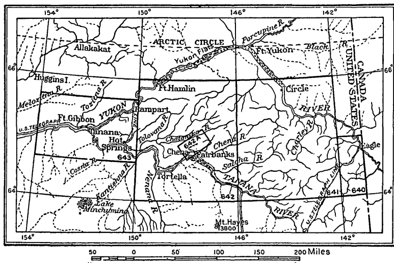
FIGURE 1.—Index map showing location of Circle quadrangle (No. 641).
