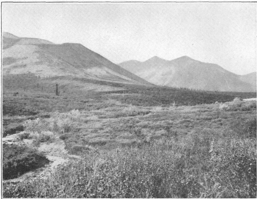
A. MORaine PARTLY DAMMING VALLEY.
