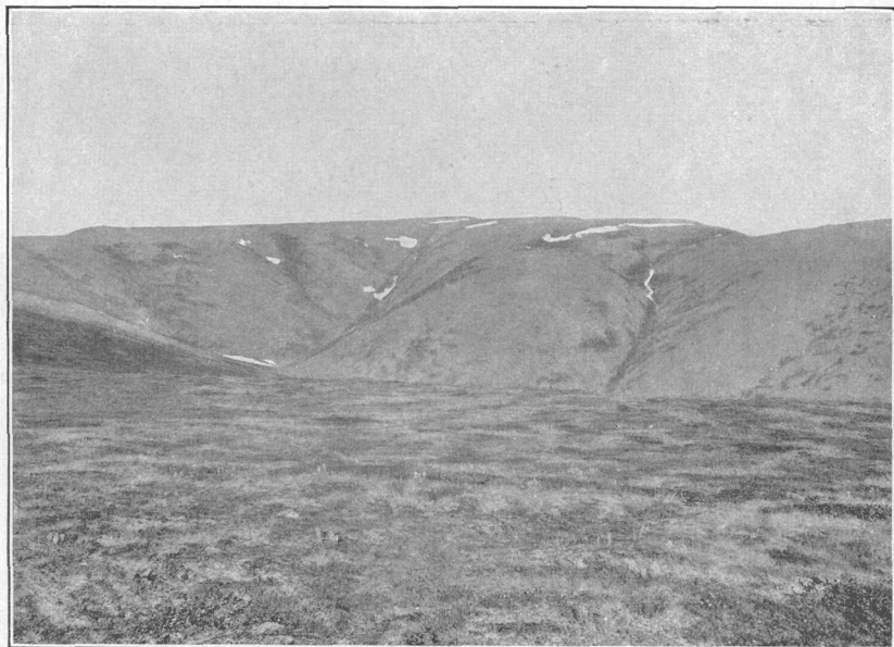
B. FLAT-TOPPED RIDGE OF QUARTZITIC SCHIST BETWEEN DAVIS AND POKER CREEKS.
