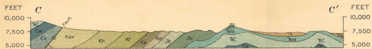
SECTION ALONG LINE C-C'
