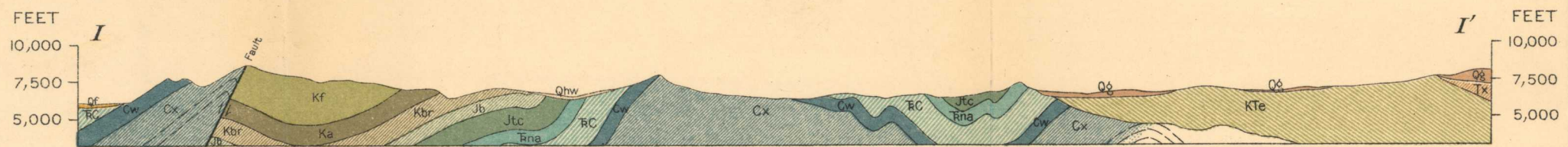
SECTION ALONG LINE I-I'
