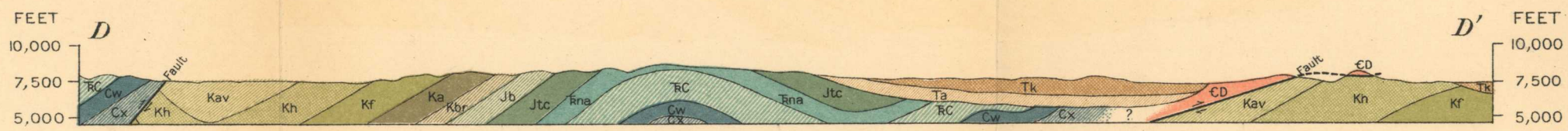
SECTION ALONG LINE D-D'
