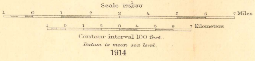
TOPOGRAPHIC MAP OF THE SANTA RITA AND PATAGONIA MOUNTAINS, ARIZONA Showing also the mining districts, settlements, camps, mines and principal prospects
