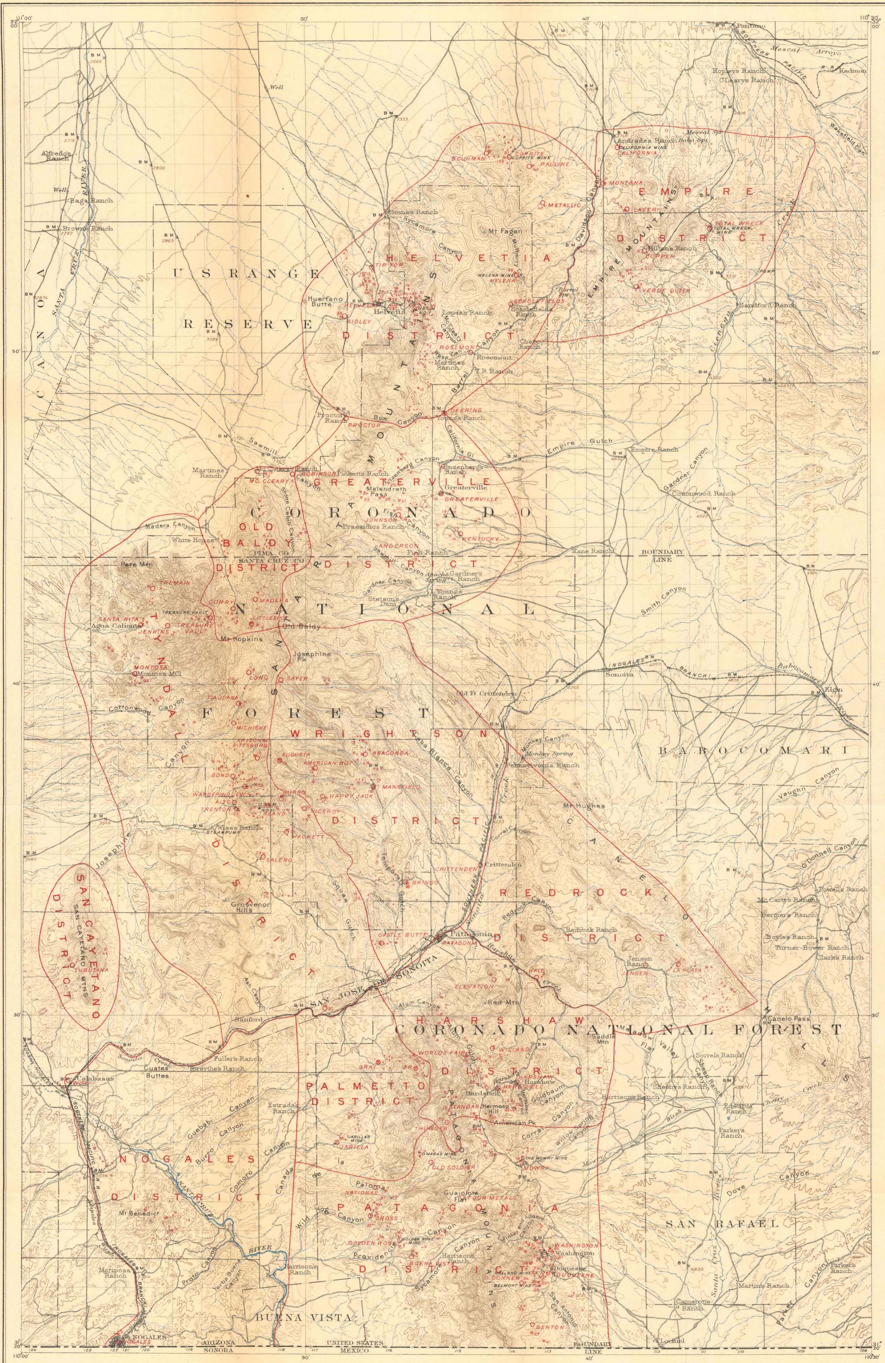
TOPOGRAPHIC MAP OF THE SANTA RITA AND PATAGONIA MOUNTAINS, ARIZONA Showing also the mining districts, settlements, camps, mines and principal prospects
