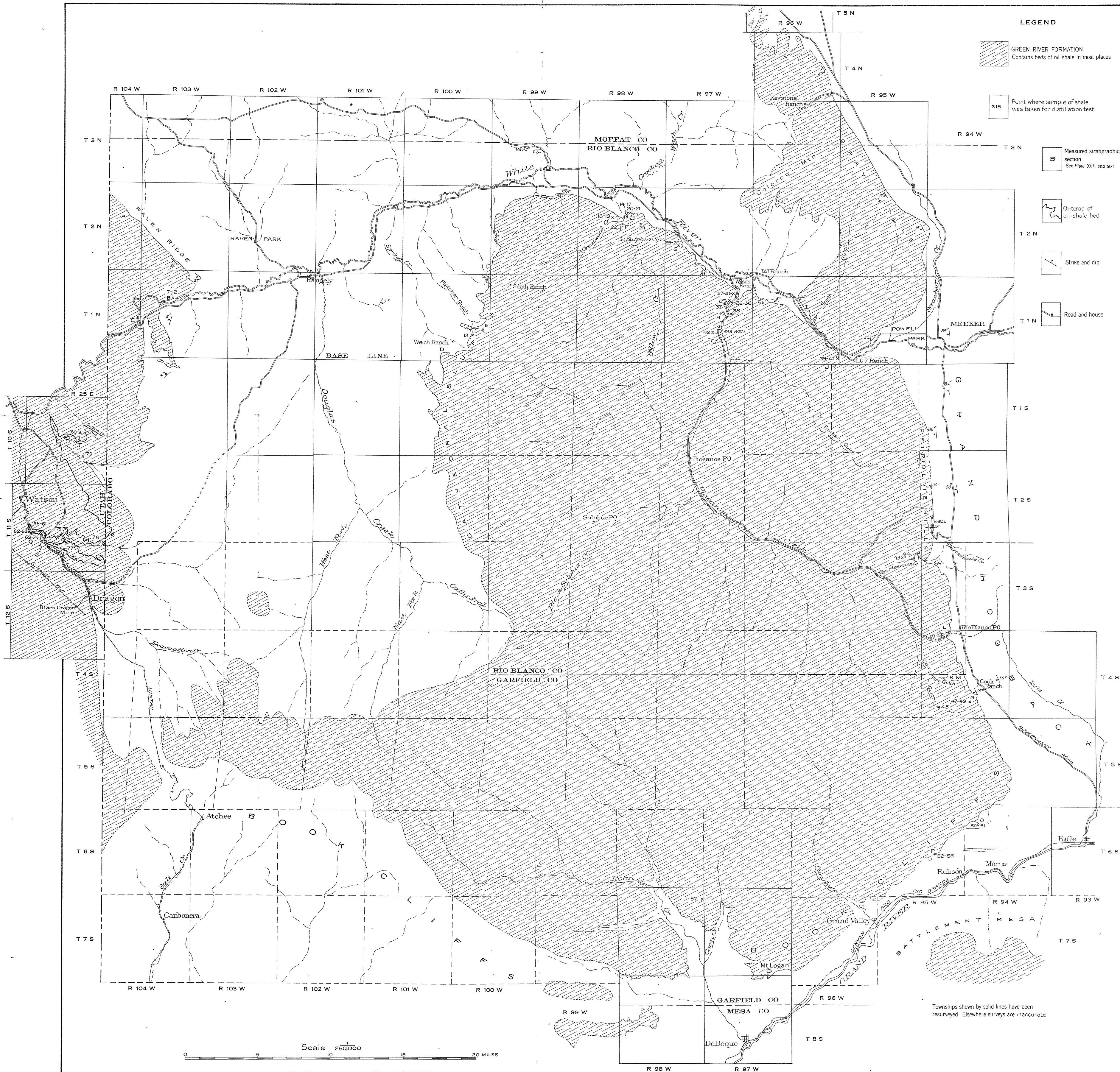
MAP OF NORTHWESTERN COLORADO AND NORTHEASTERN UTAH SHOWING AREAS OF GREEN RIVER FORMATION By Dean E. Winchester
