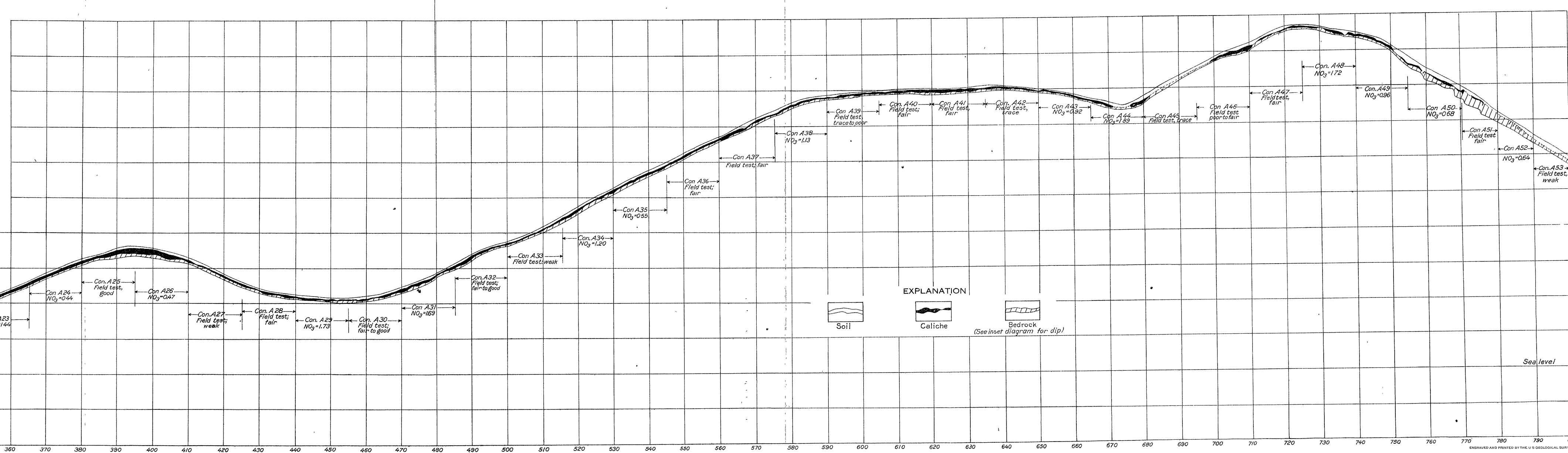
PROFILE OF LONG TRENCH A, CONFIDENCE HILLS
