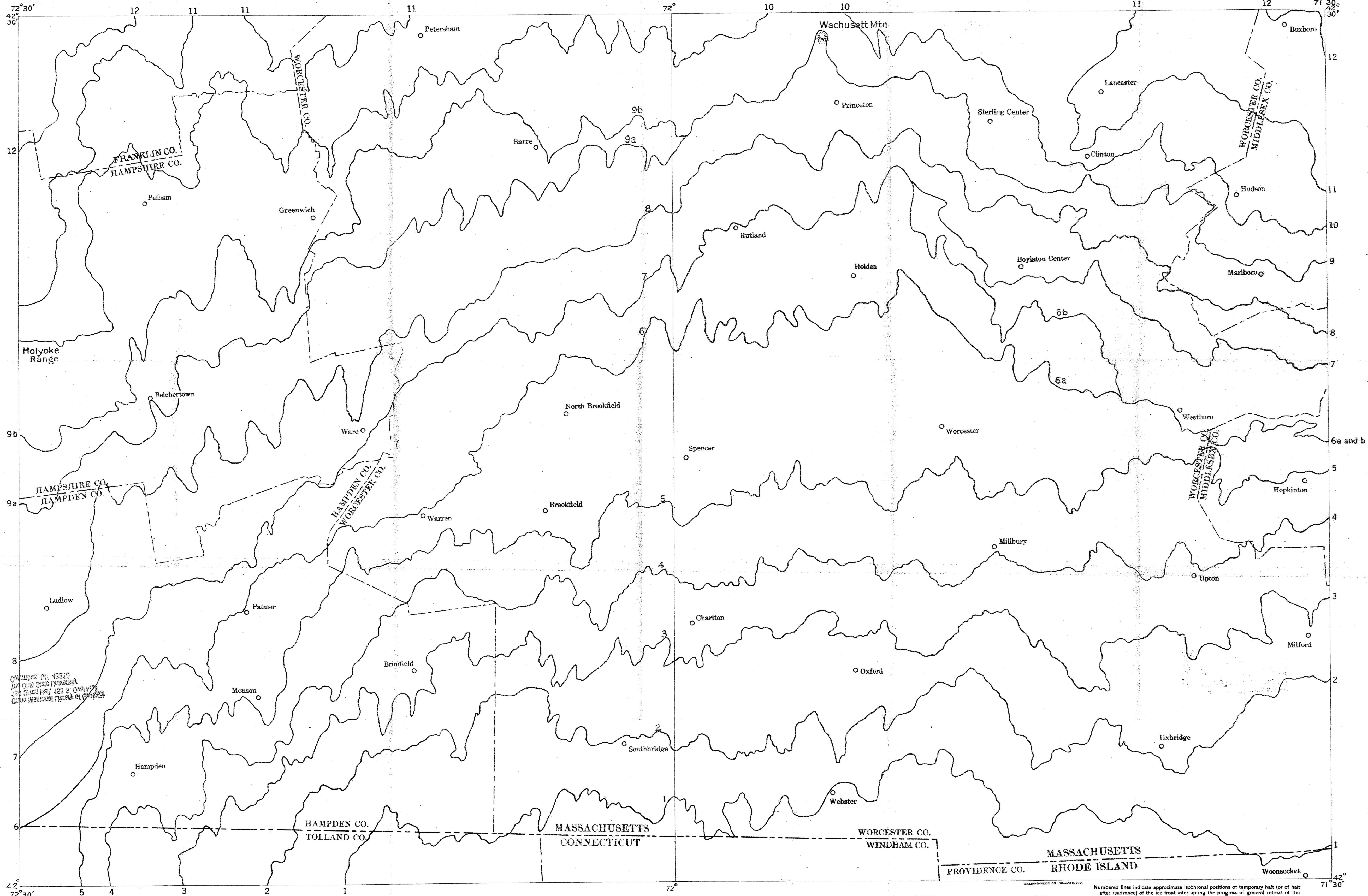
HYPOTHETICAL STAGES OF RETREAT OF THE GLACIAL MARGIN IN WARE AND QUINSIGAMOND QUADRANGLES, MASSACHUSETTS
