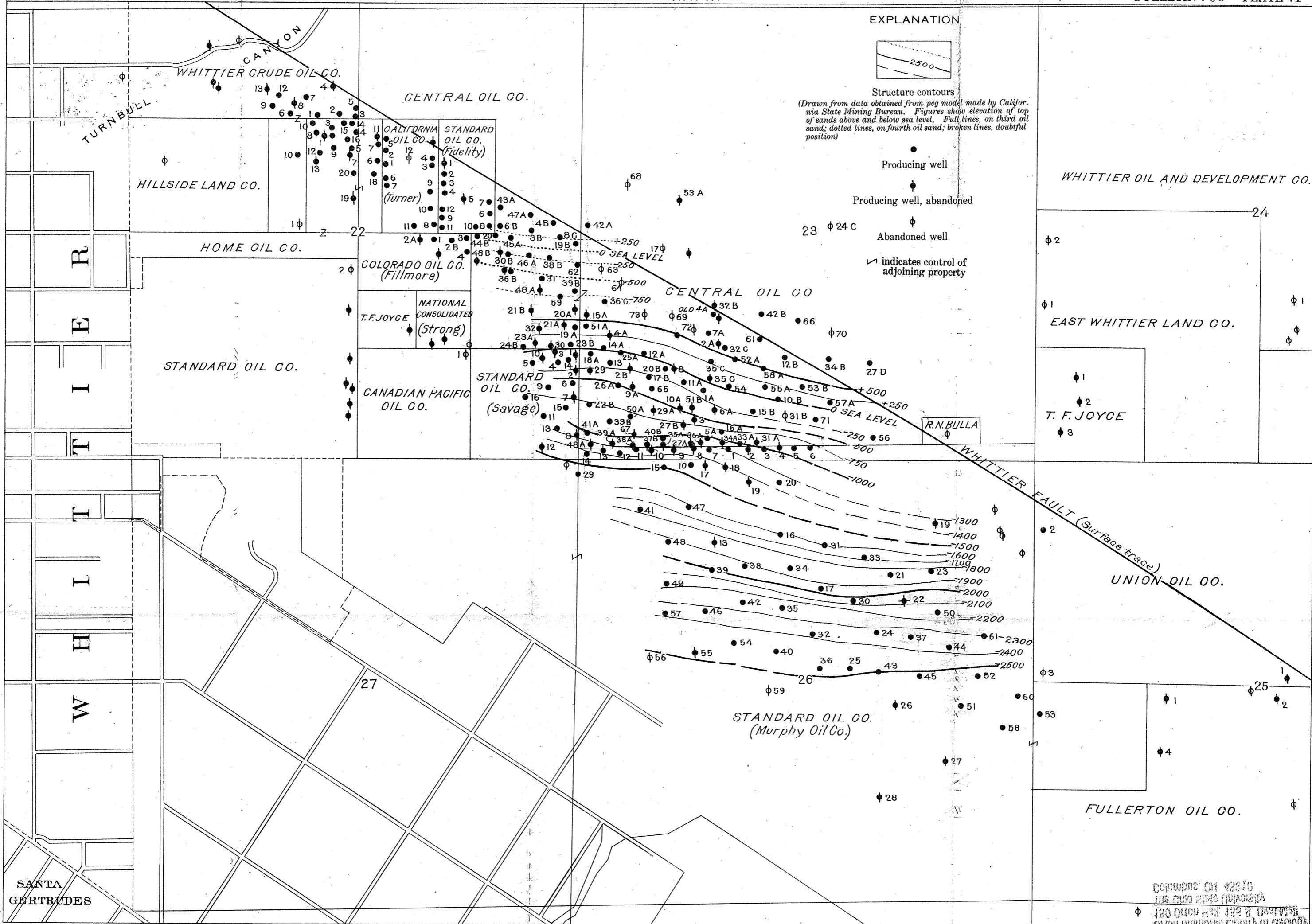
MAP SHOWING GEOLOGIC STRUCTURE OF PART OF WHITTIER OIL FIELD, CALIFORNIA
