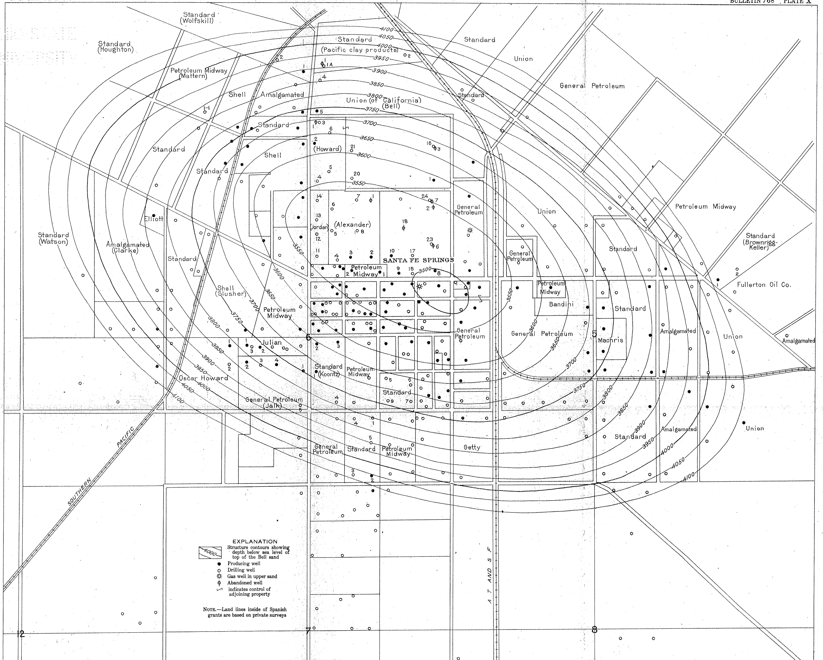
MAP SHOWING STRUCTURE OF SANTA FE SPRINGS FIELD, CALIFORNIA
