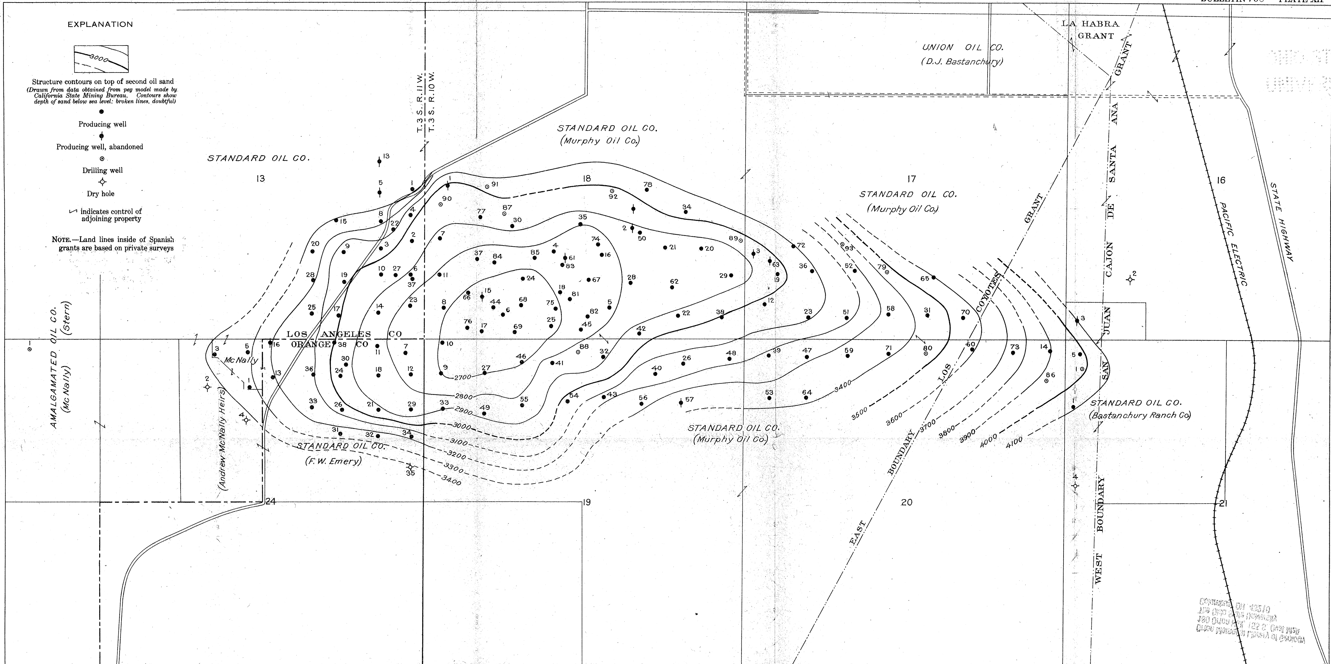
MAP SHOWING GEOLOGIC STRUCTURE OF WEST COYOTE HILLS OIL FIELD, CALIFORNIA
