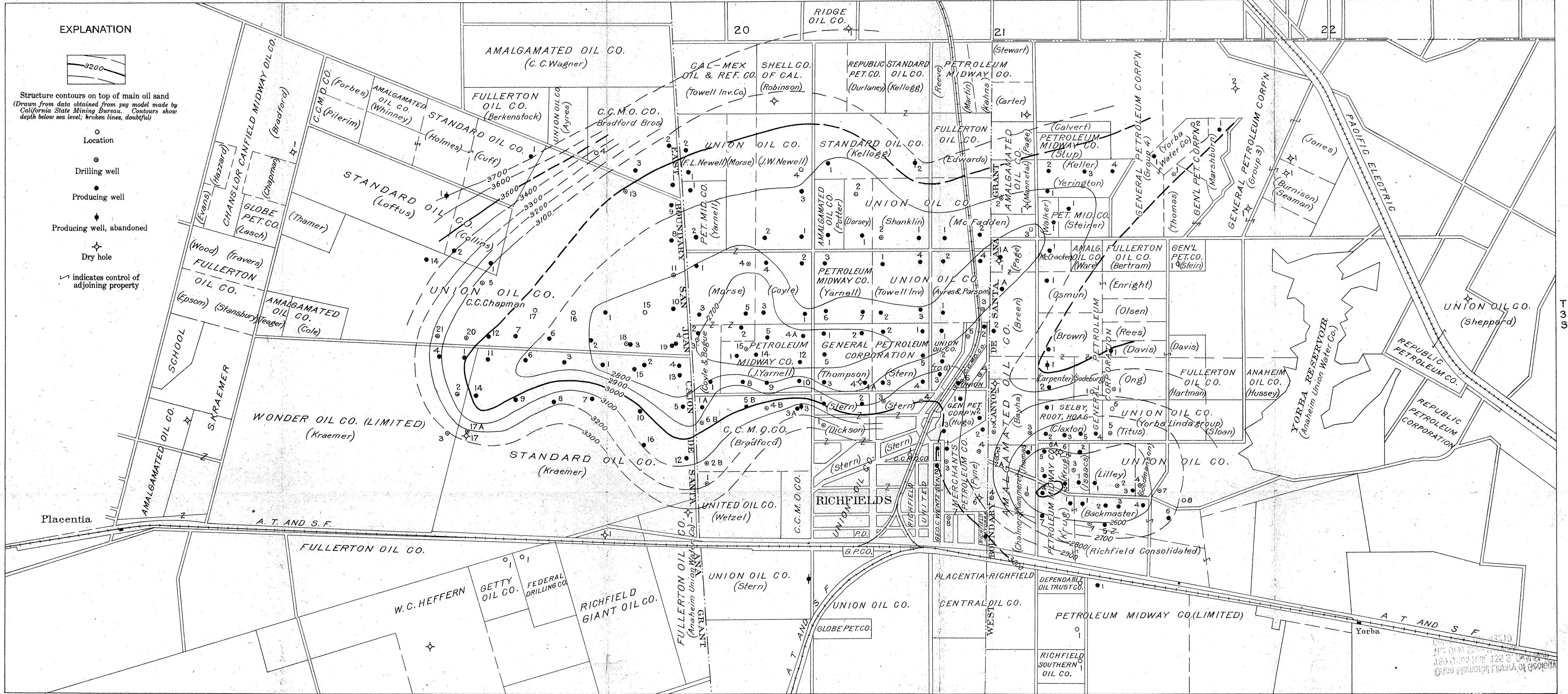
MAP SHOWING GEOLOGIC STRUCTURE OF RICHFIELDS OIL FIELD, CALIFORNIA
