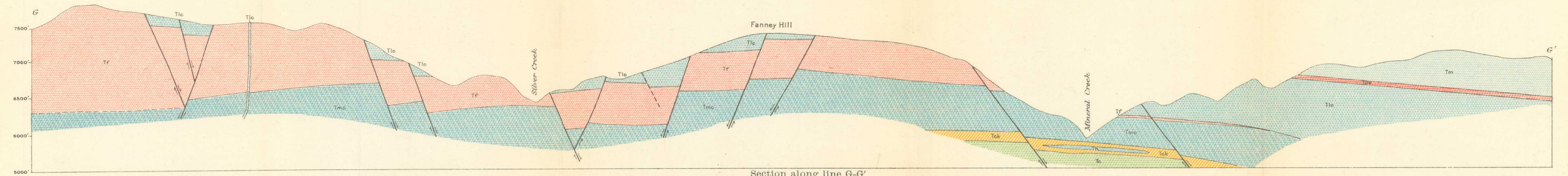
Section along line G-G'
