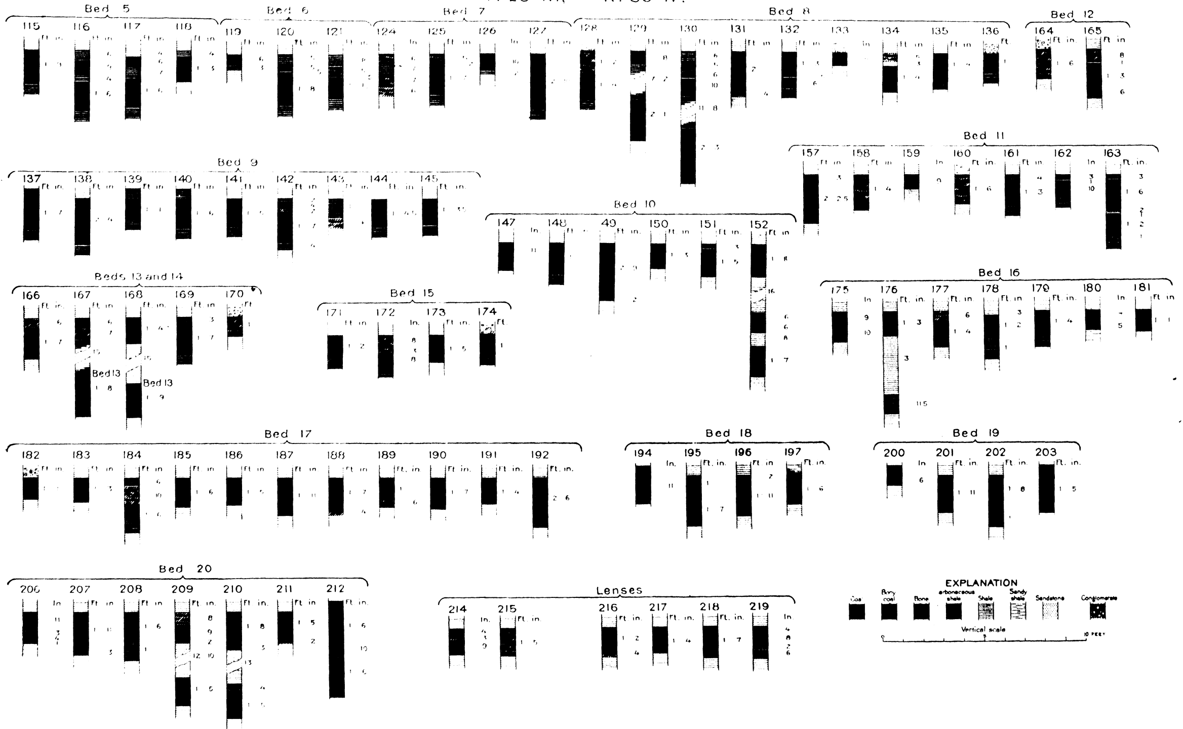
SECTIONS OF COAL BEDS IN T. 23 N., R. 85 W.
