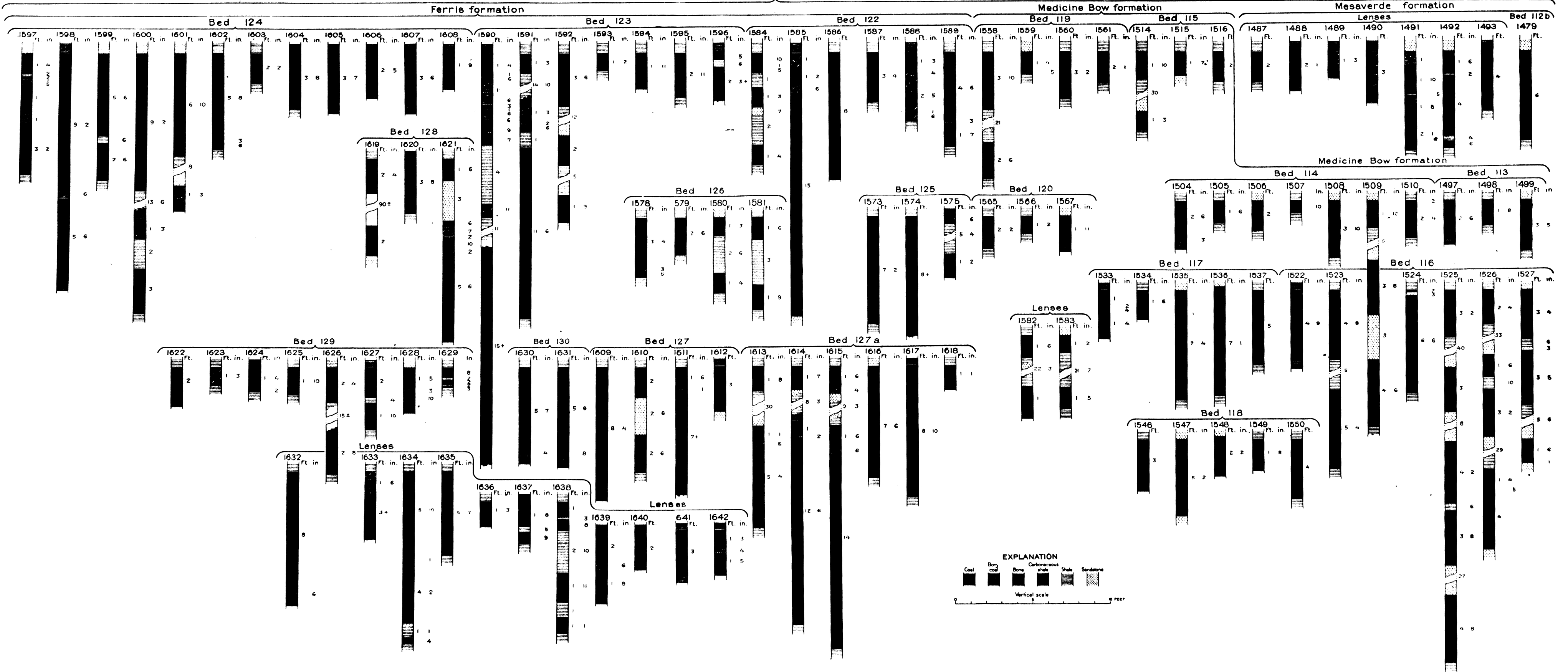
SECTIONS OF COAL BEDS IN T. 24 N., R. 83 W.
