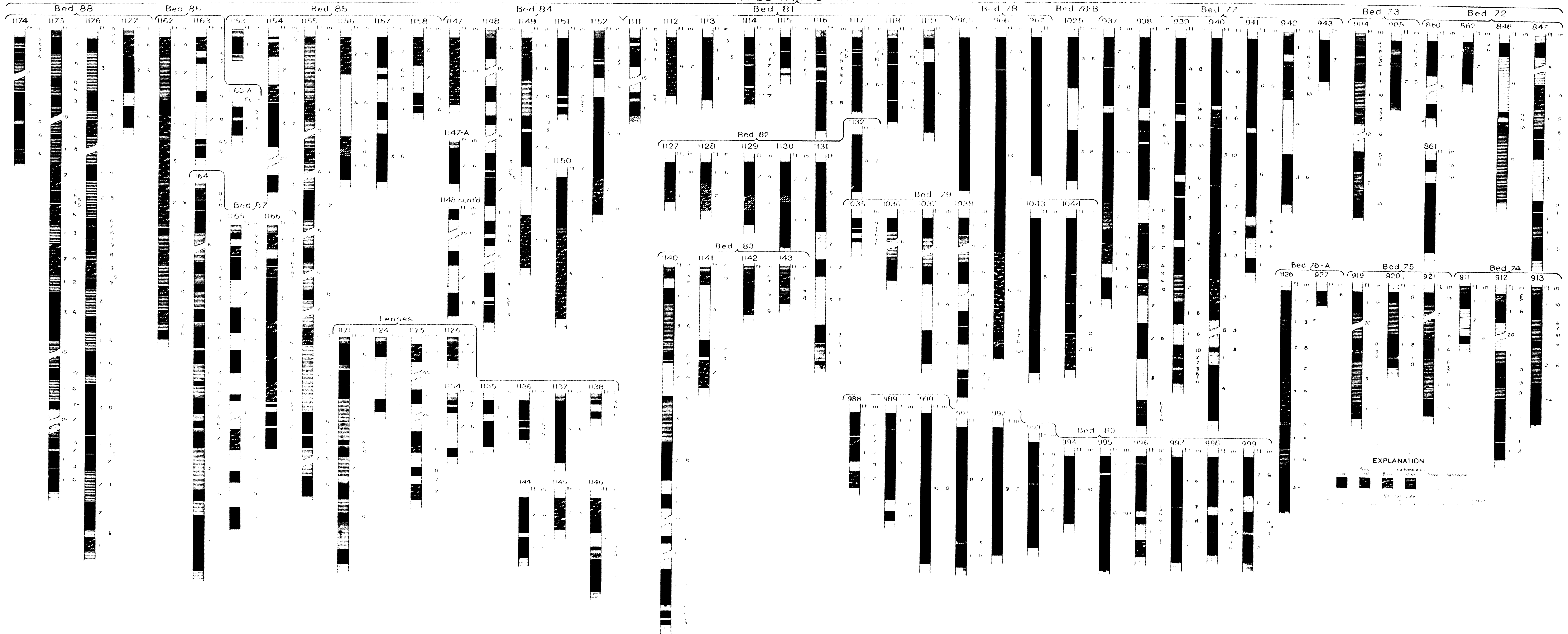
SECTIONS OF COAL BEDS IN T. 23 N., R. 81 W.
