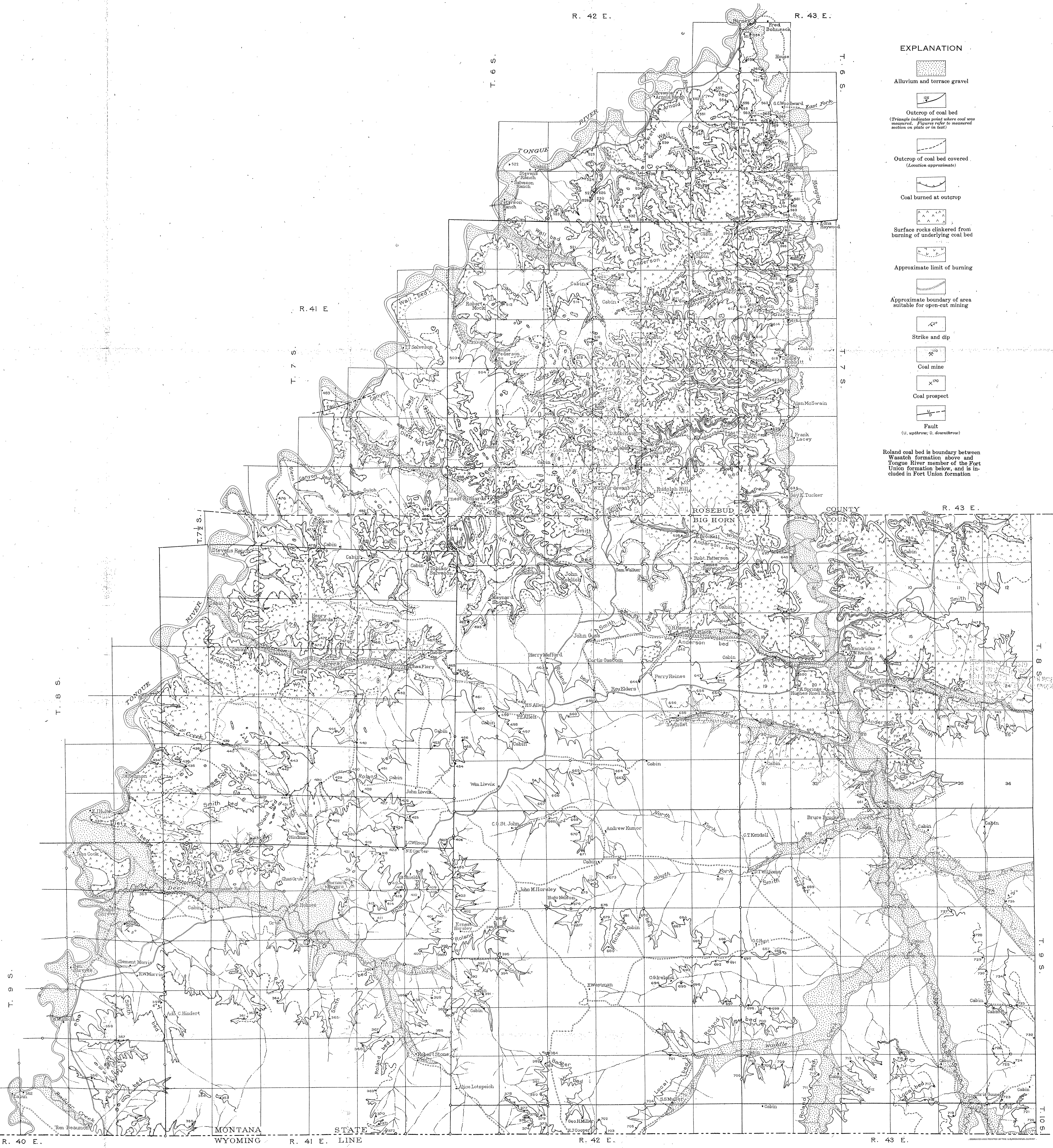
MAP OF THE EASTERN PART OF THE NORTHWARD EXTENSION OF THE SHERIDAN COAL FIELD, ROSEBUD AND BIG HORN COUNTIES, MONTANA
