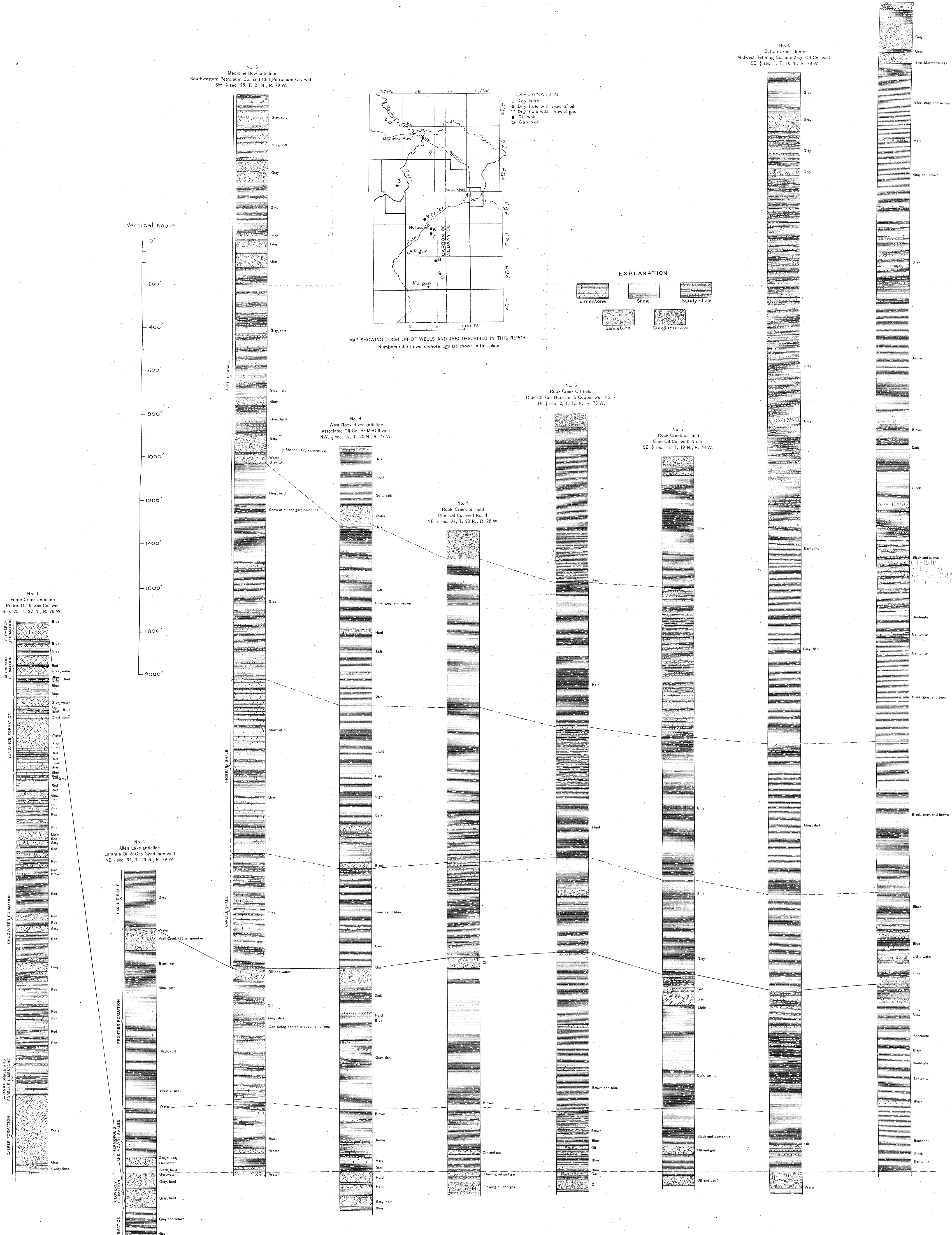
REPRESENTATIVE GRAPHIC WELL LOGS OF THE ROCK CREEK AND ADJOINING AREAS, WYOMING
