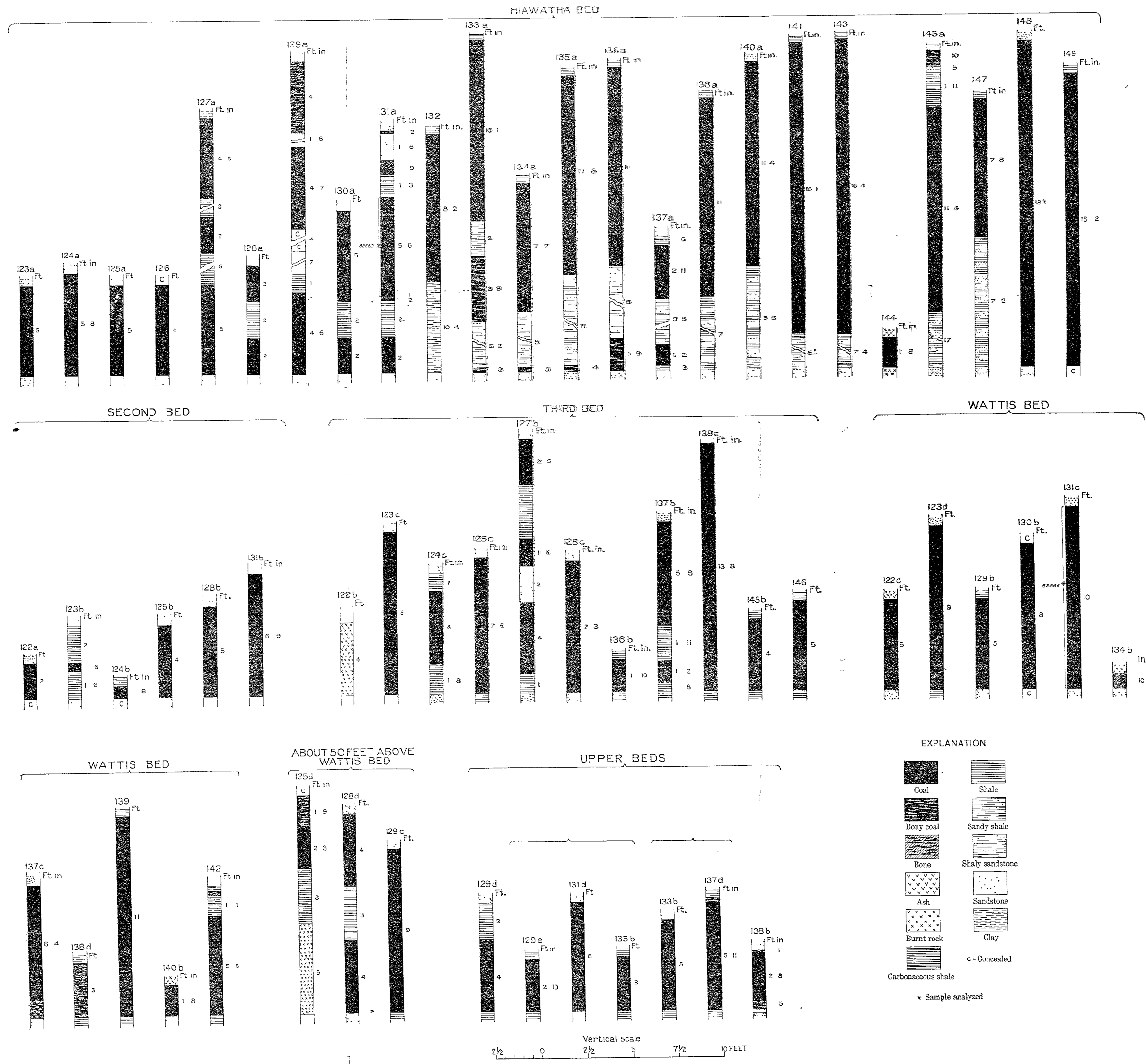
SECTIONS OF COAL BEDS AND COLUMNAR SECTIONS, HIAWATHA AREA
