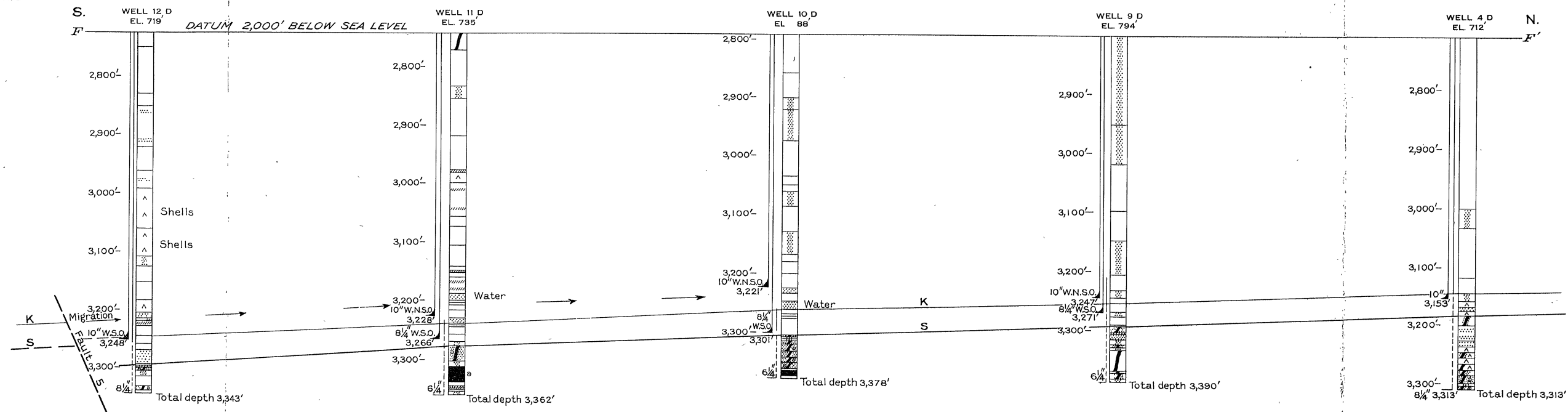
A. SECTION ALONG LINE F-F' OF PLATE 13
