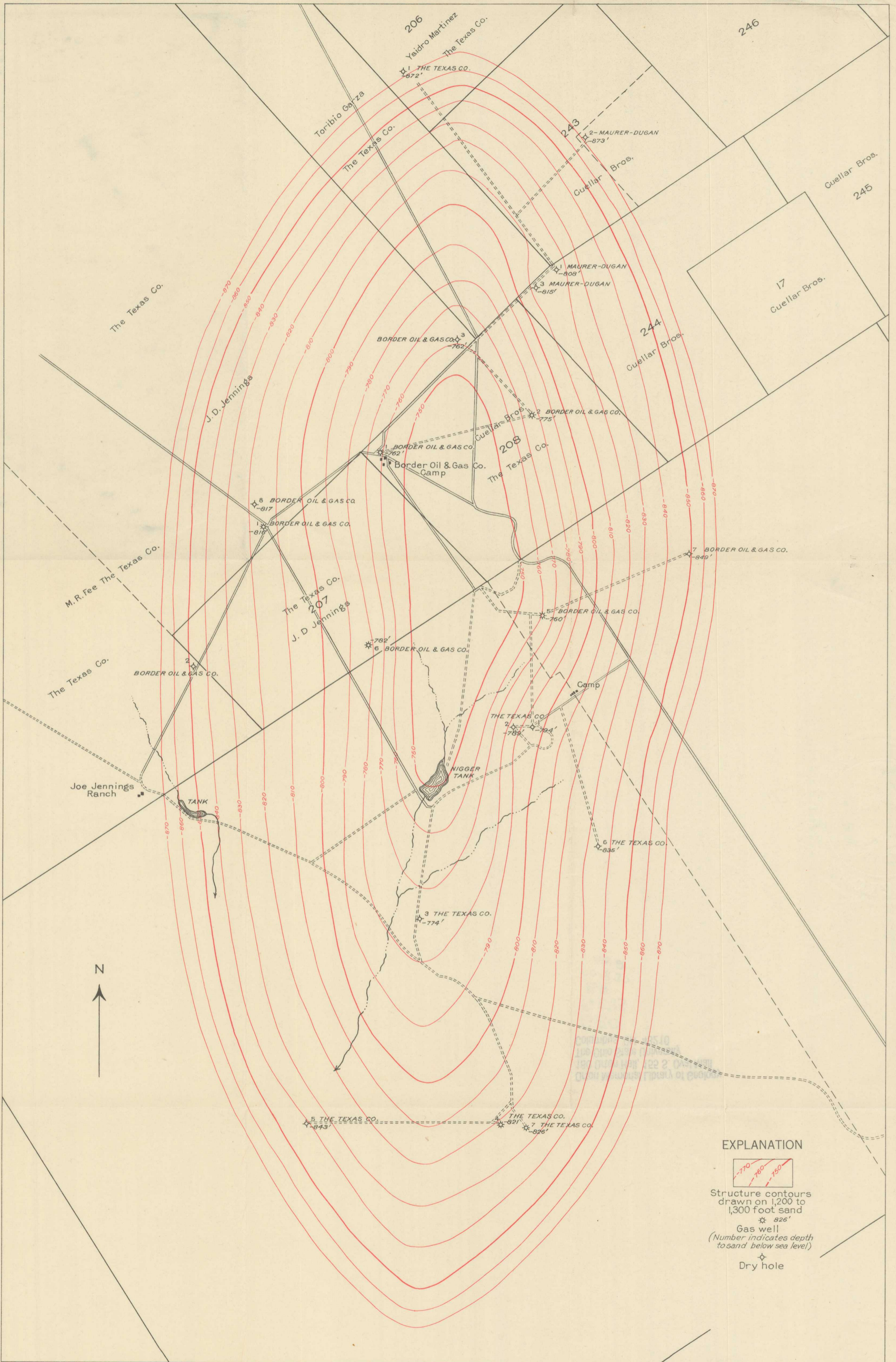
MAP OF THE JENNINGS GAS FIELD, LOWER RIO GRANDE REGION, ZAPATA COUNTY, TEXAS, SHOWING WELLS AND STRUCTURE CONTOURS
