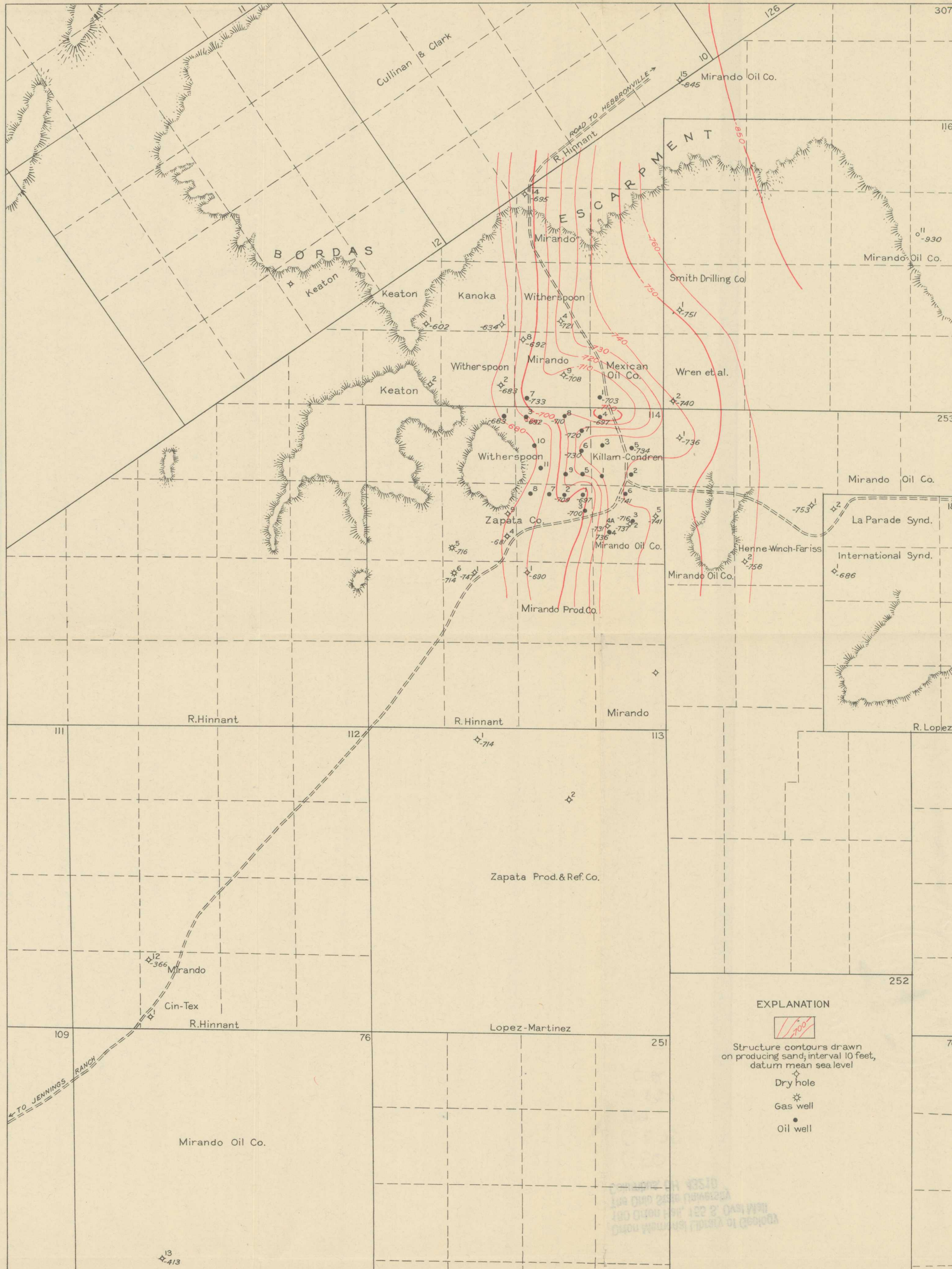
MAP OF THE MIRANDO VALLEY OIL AND GAS FIELD, LOWER RIO GRANDE REGION, SOUTHWEST TEXAS, SHOWING WELLS AND STRUCTURE CONTOURS
