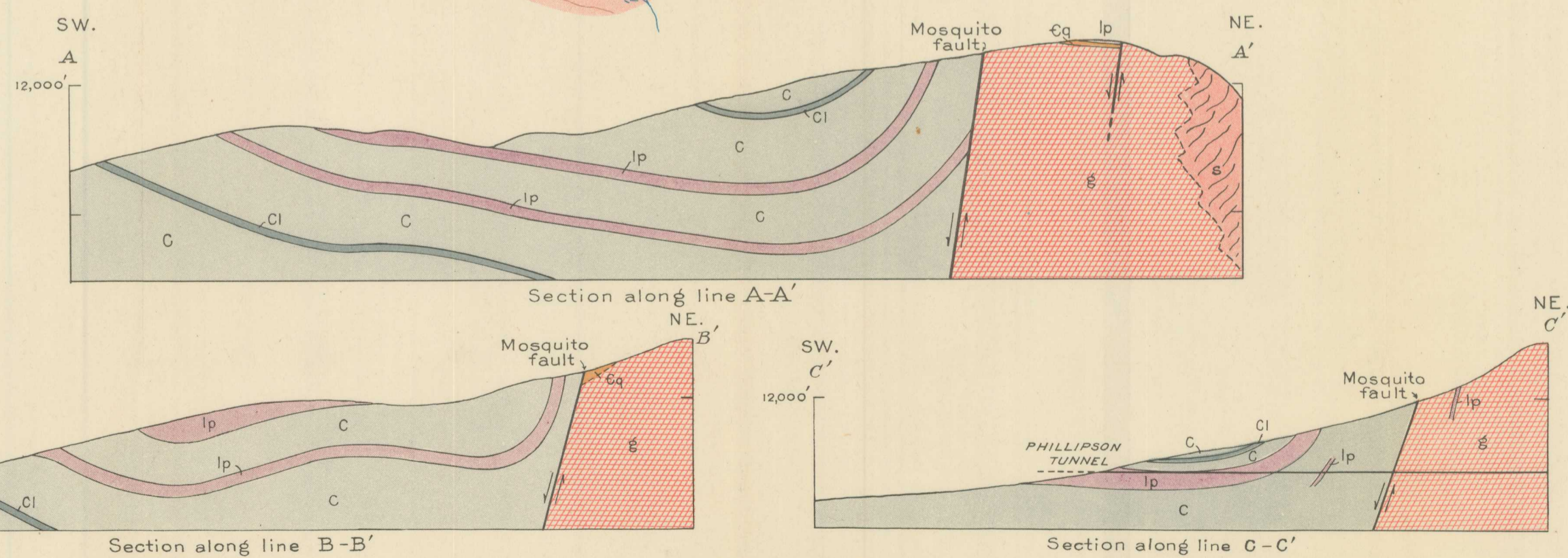
GEOLOGIC MAP AND SECTIONS OF CLIMAX MINING DISTRICT, COLORADO Sections A-A' and B-B' are partly diagrammatic; section C-C' shows structure found in the Phillipson tunnel, where only one syncline is present
